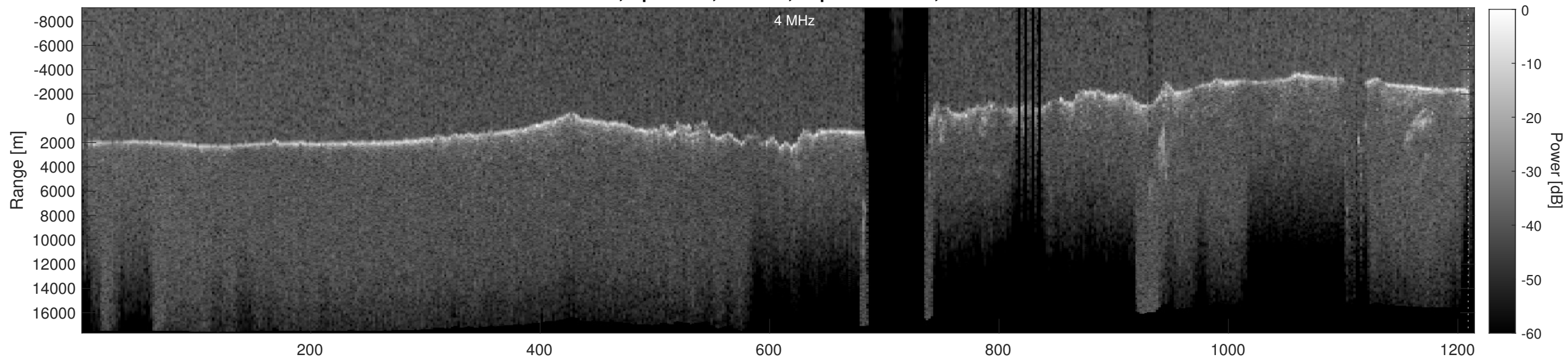
Orbit 15707, Depth-Corrected Cluttergram
