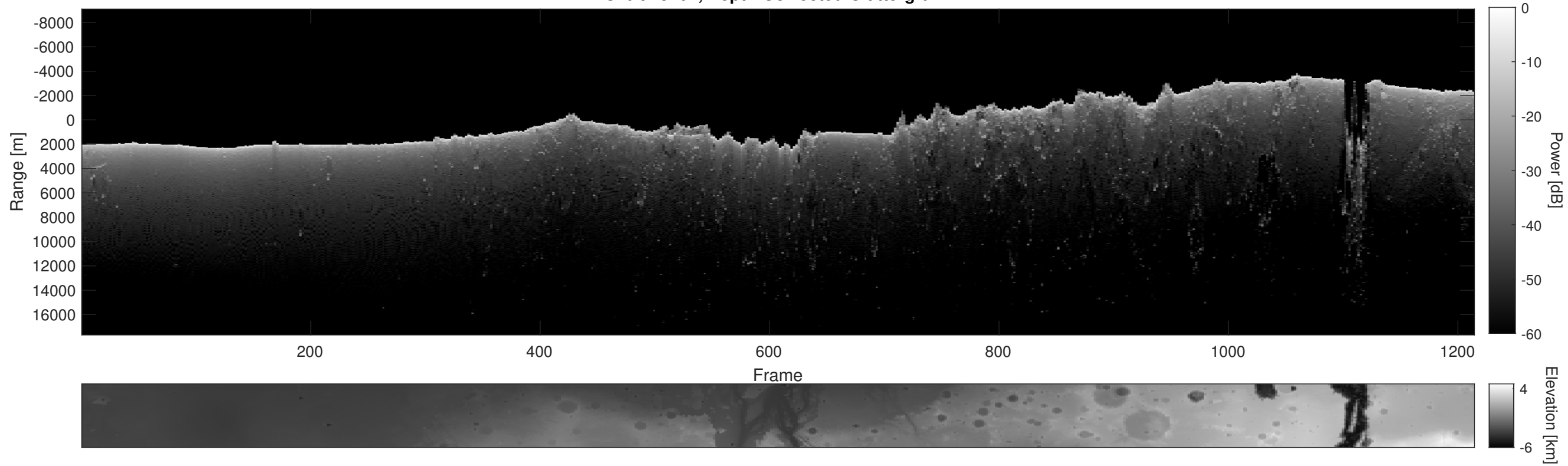
Orbit 15707, Depth-Corrected Cluttergram
