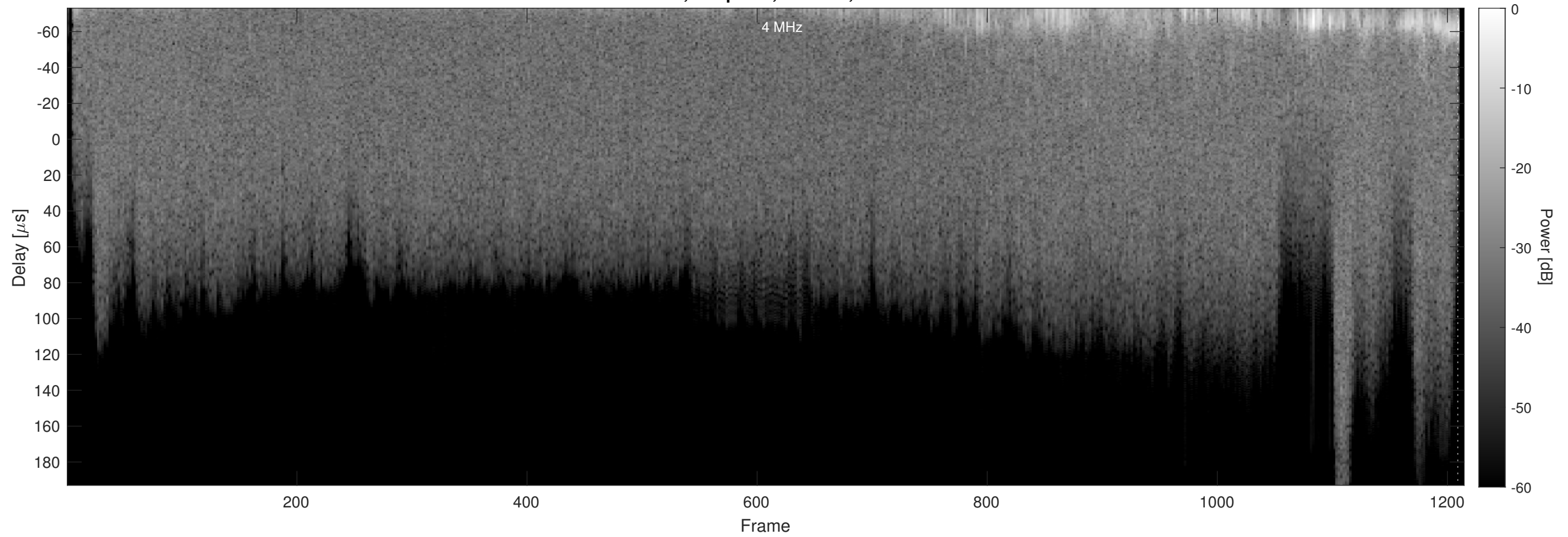
Orbit 15709, Chapman, Window, Channel 2
