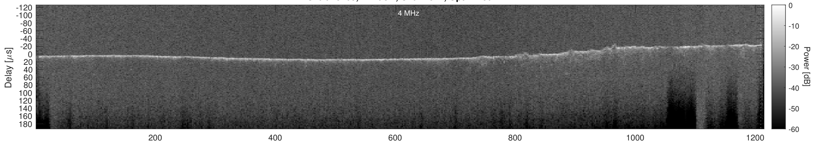
Orbit 15709, Cluttergram
