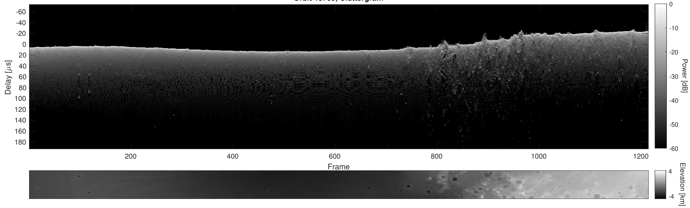
Orbit 15709, Cluttergram
