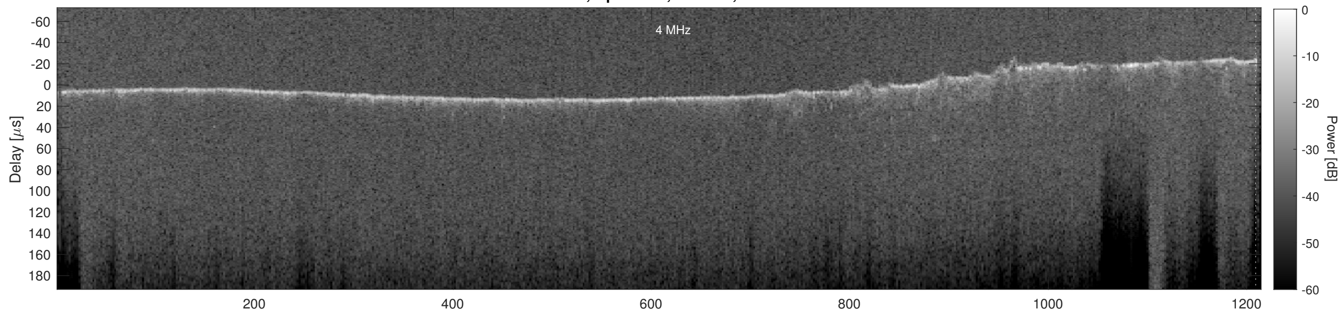
Orbit 15709, Cluttergram
