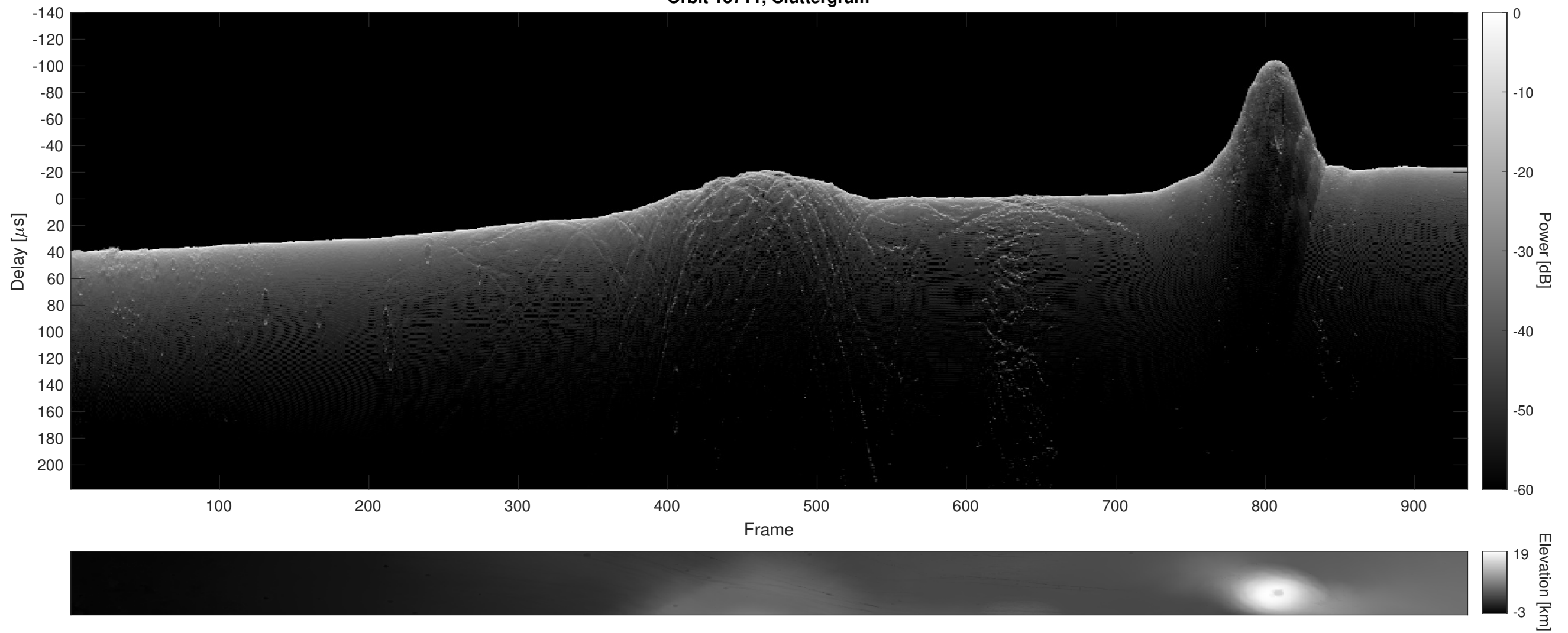
Orbit 15711, Cluttergram
