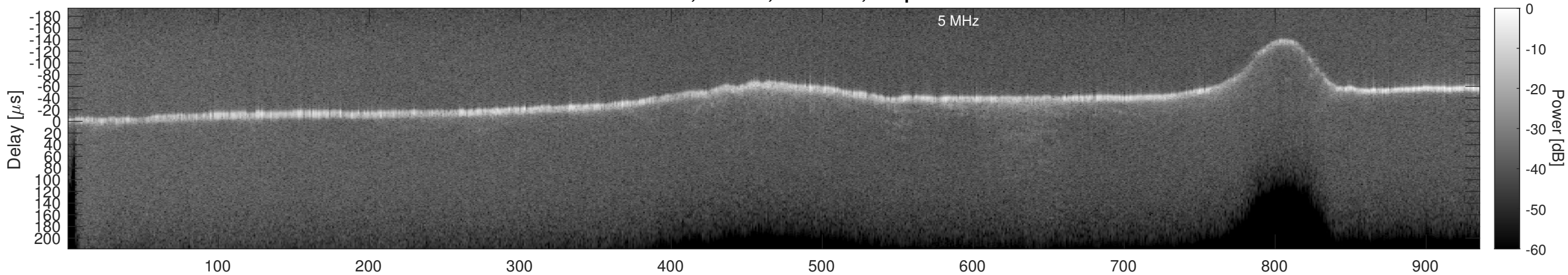
Orbit 15711, Window, Channel 1, Optimized
