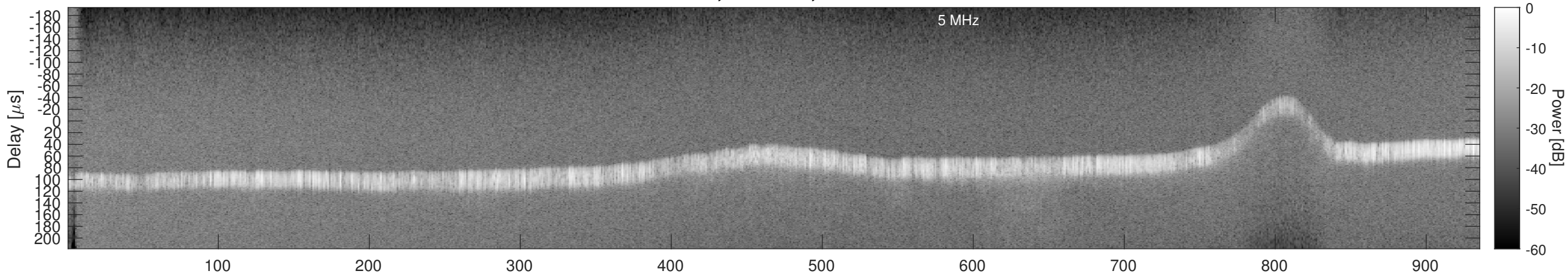
Orbit 15711, Window, Channel 1, Chapman
