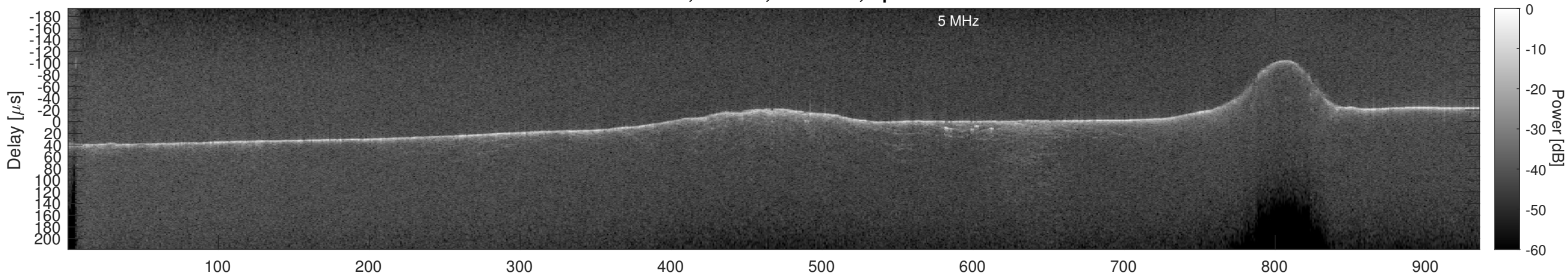
Orbit 15711, Cluttergram
