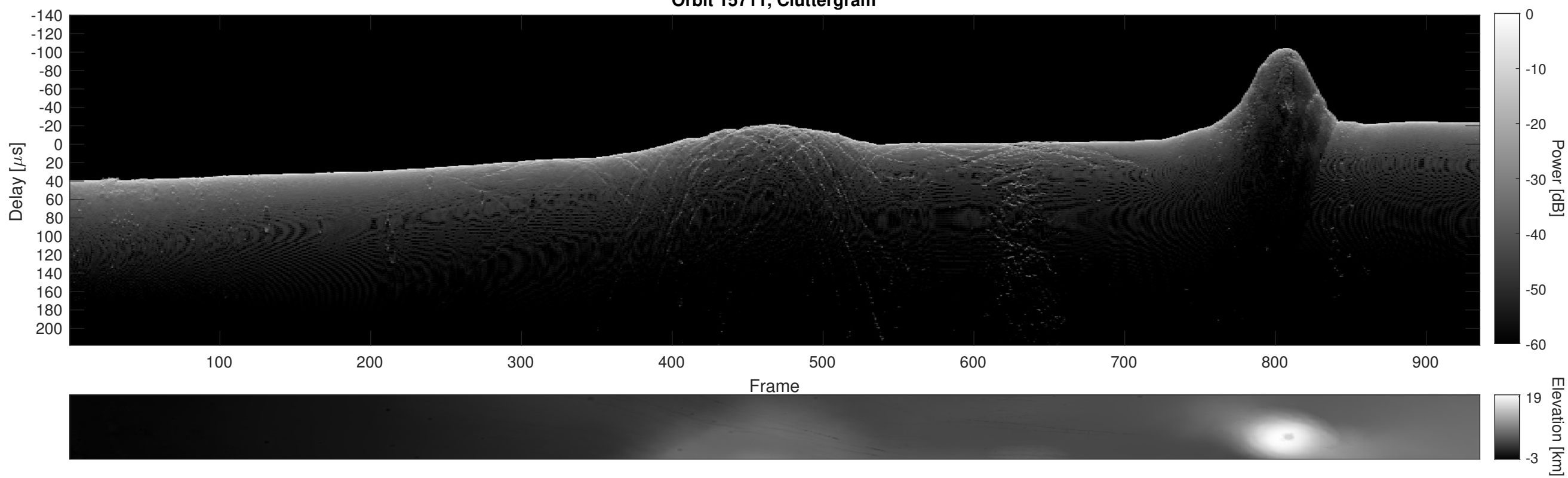
Orbit 15711, Cluttergram
