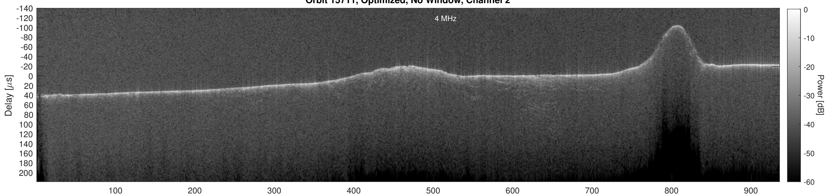
Orbit 15711, Cluttergram
