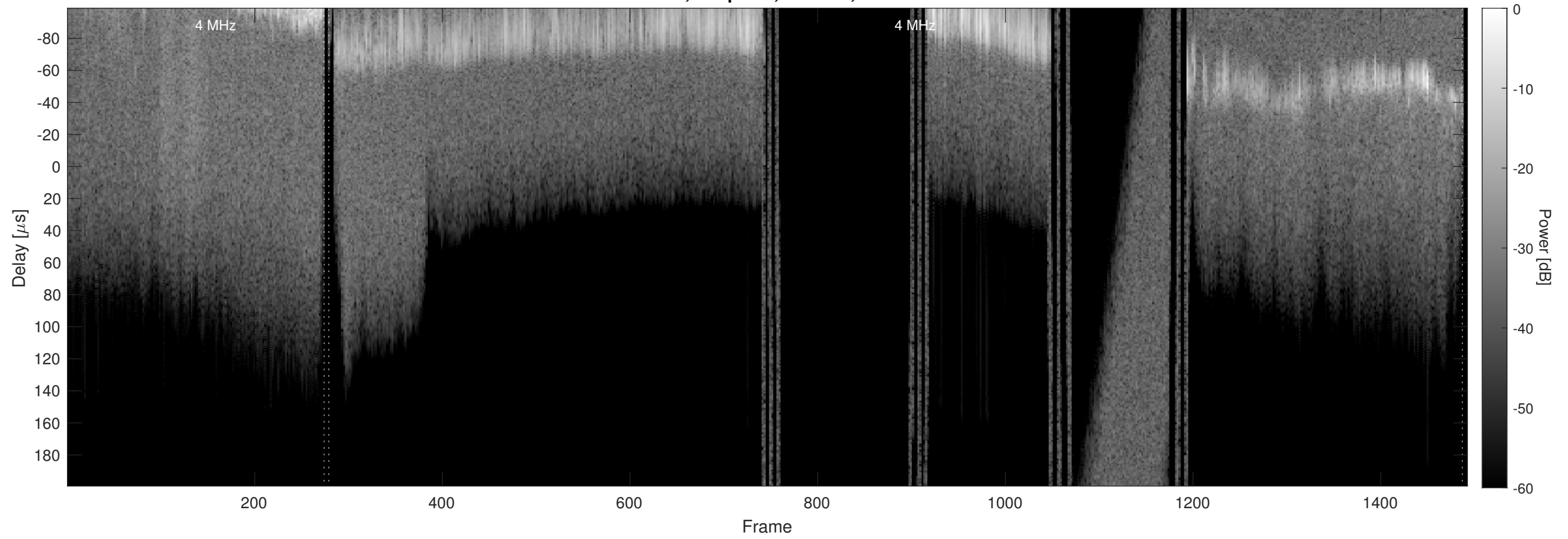
Orbit 15712, Chapman, Window, Channel 2
