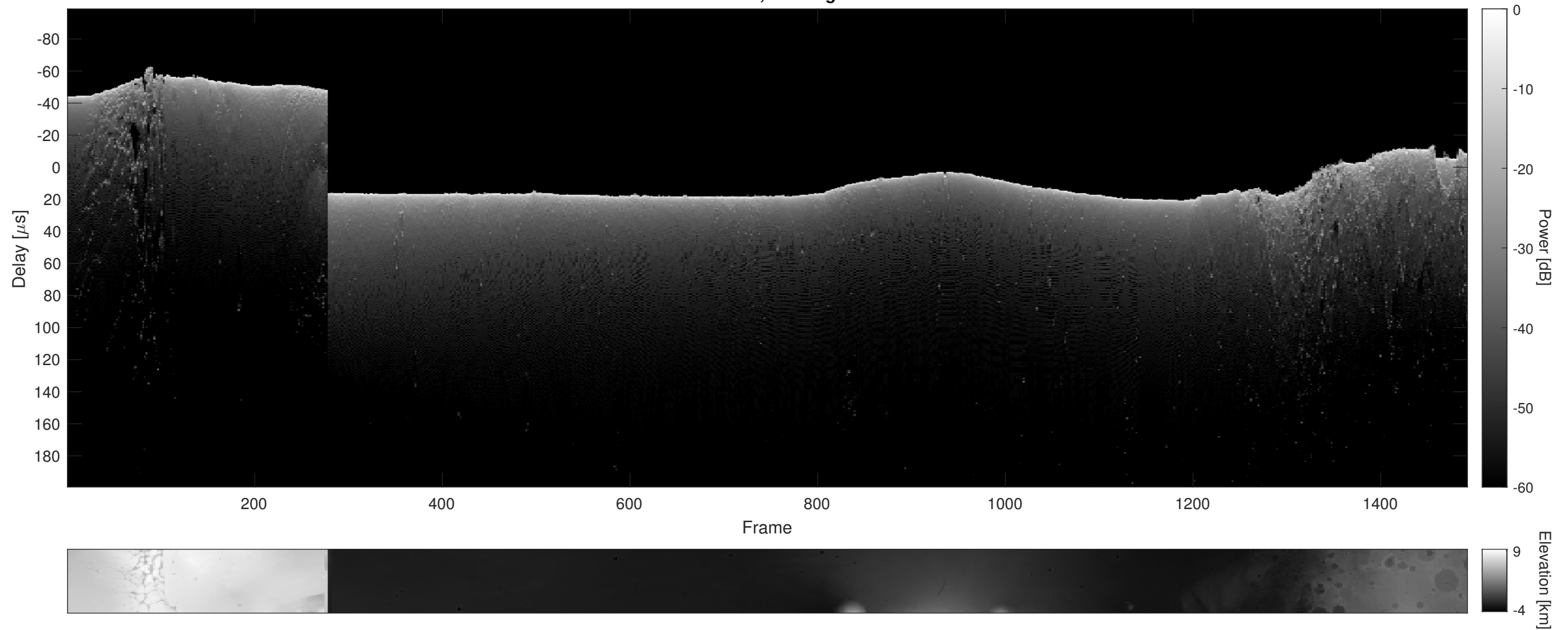
Orbit 15712, Cluttergram
