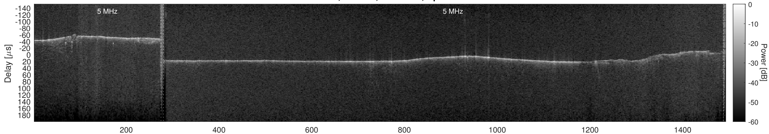
Orbit 15712, Cluttergram
