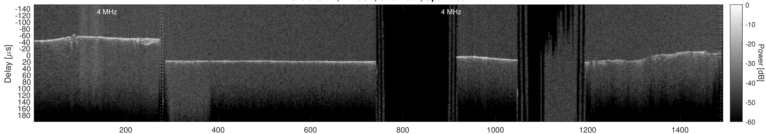
Orbit 15712, Cluttergram
