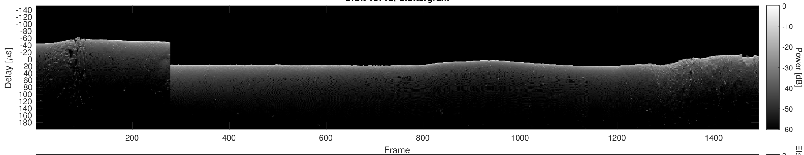
Orbit 15712, Cluttergram
