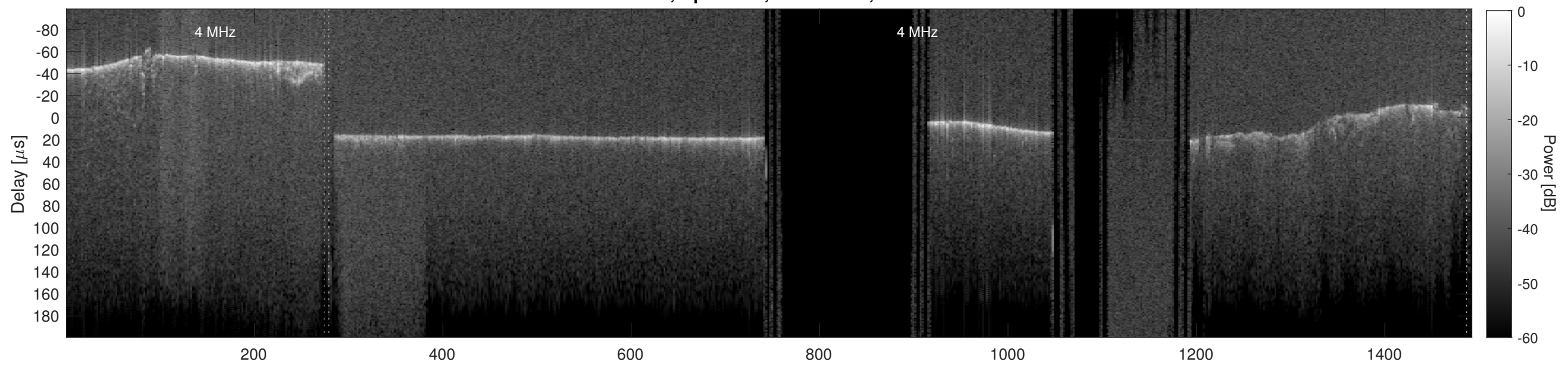
Orbit 15712, Cluttergram
