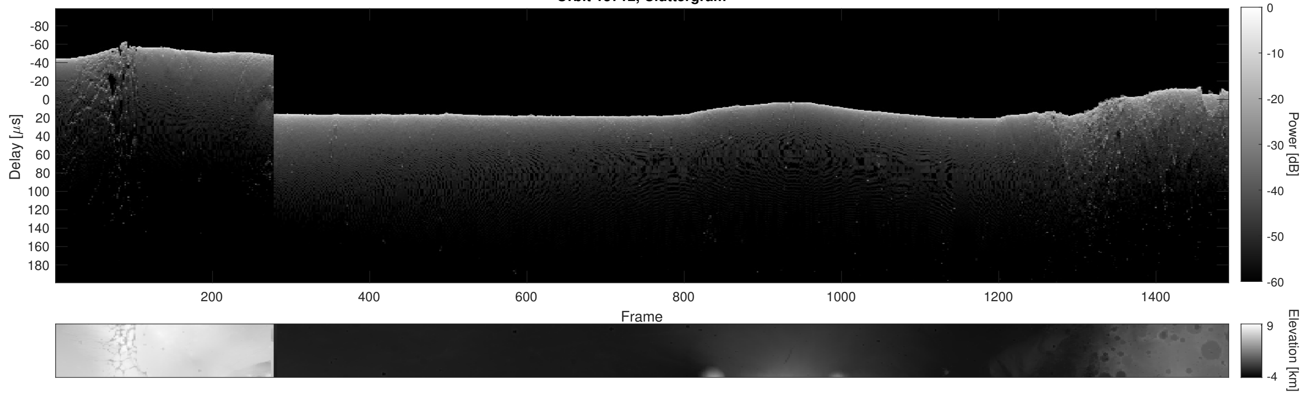
Orbit 15712, Cluttergram
