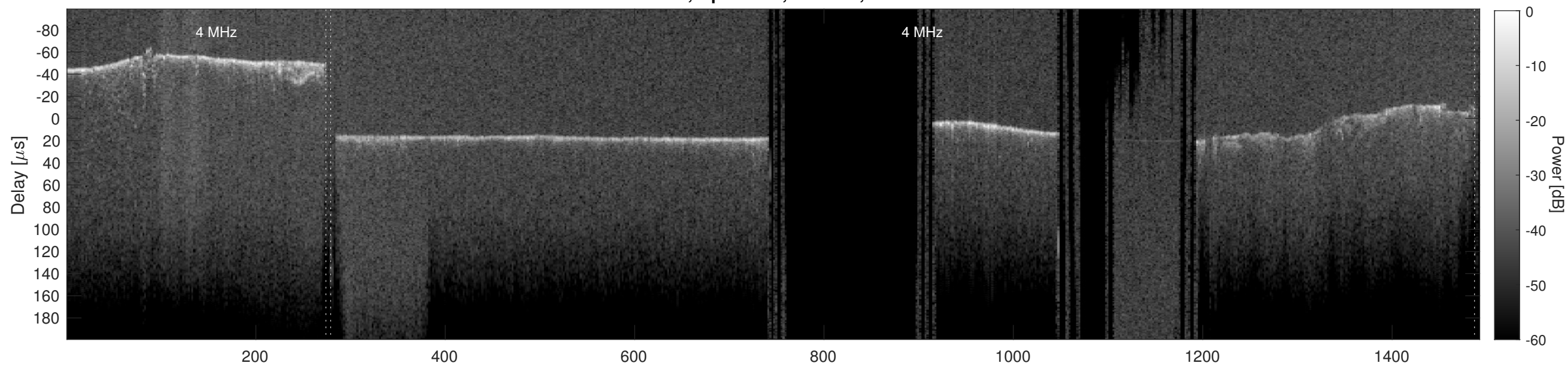
Orbit 15712, Cluttergram
