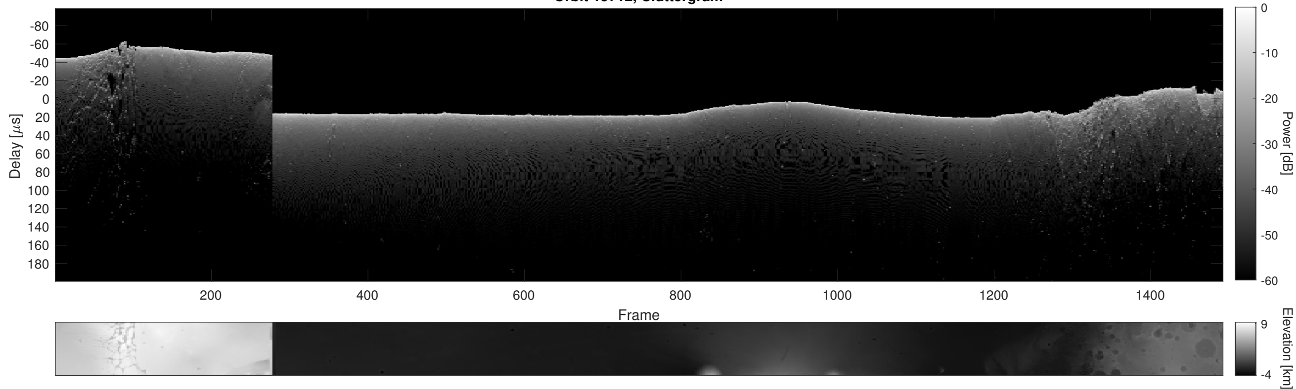
Orbit 15712, Cluttergram
