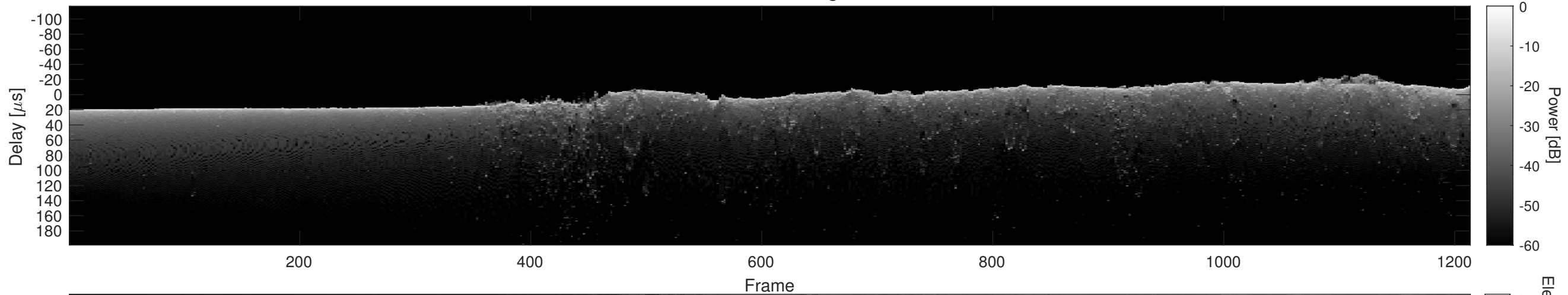
Orbit 15713, Cluttergram
