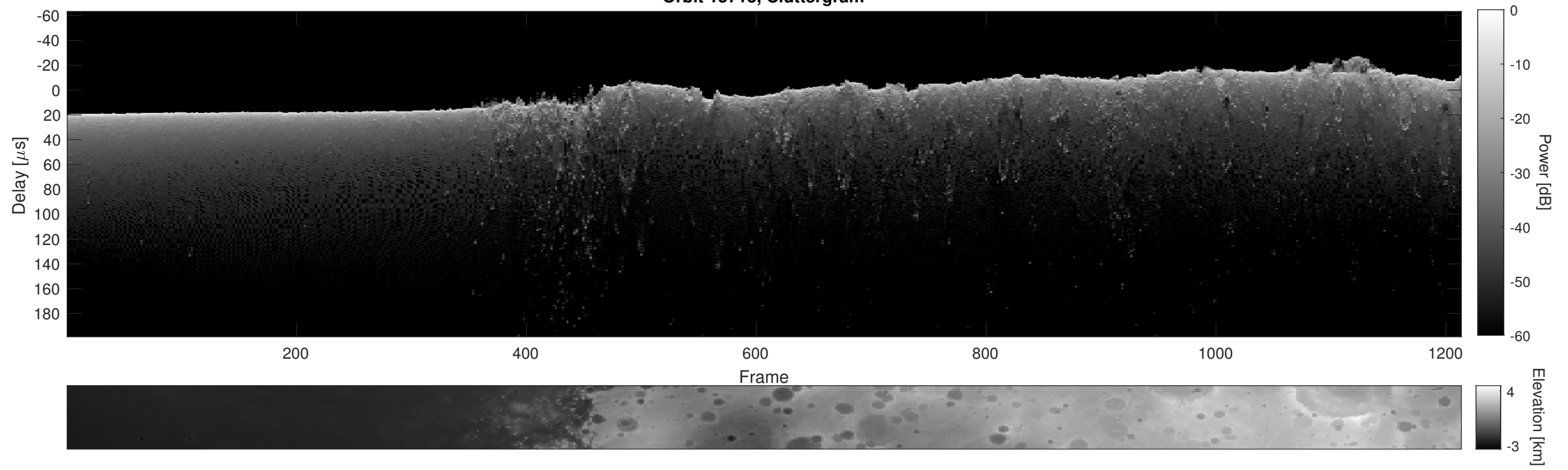
Orbit 15713, Cluttergram
