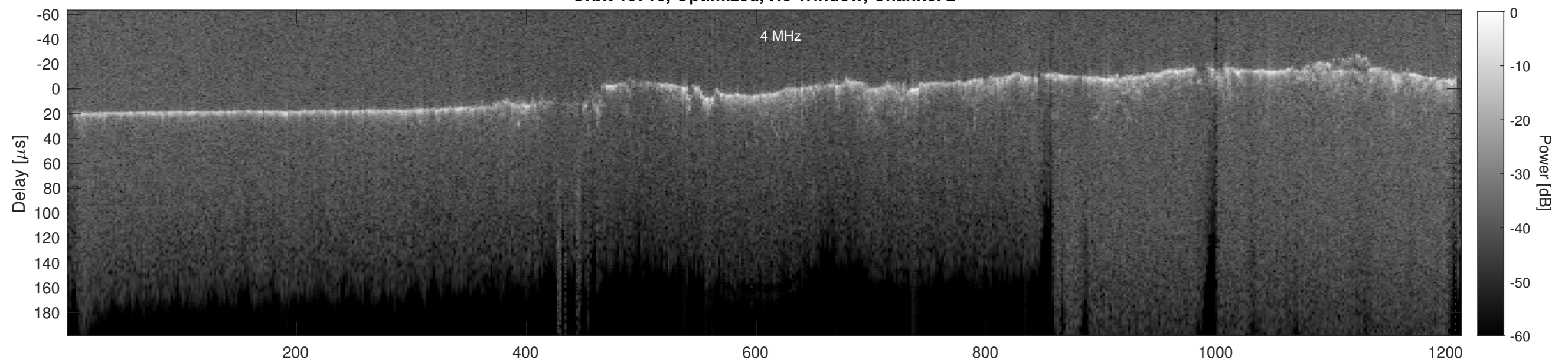
Orbit 15713, Cluttergram
