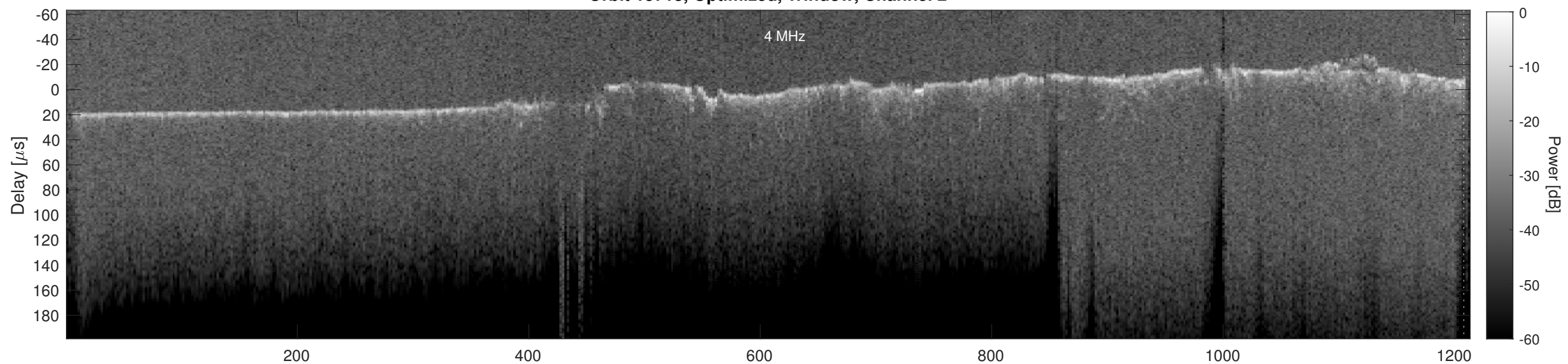
Orbit 15713, Cluttergram
