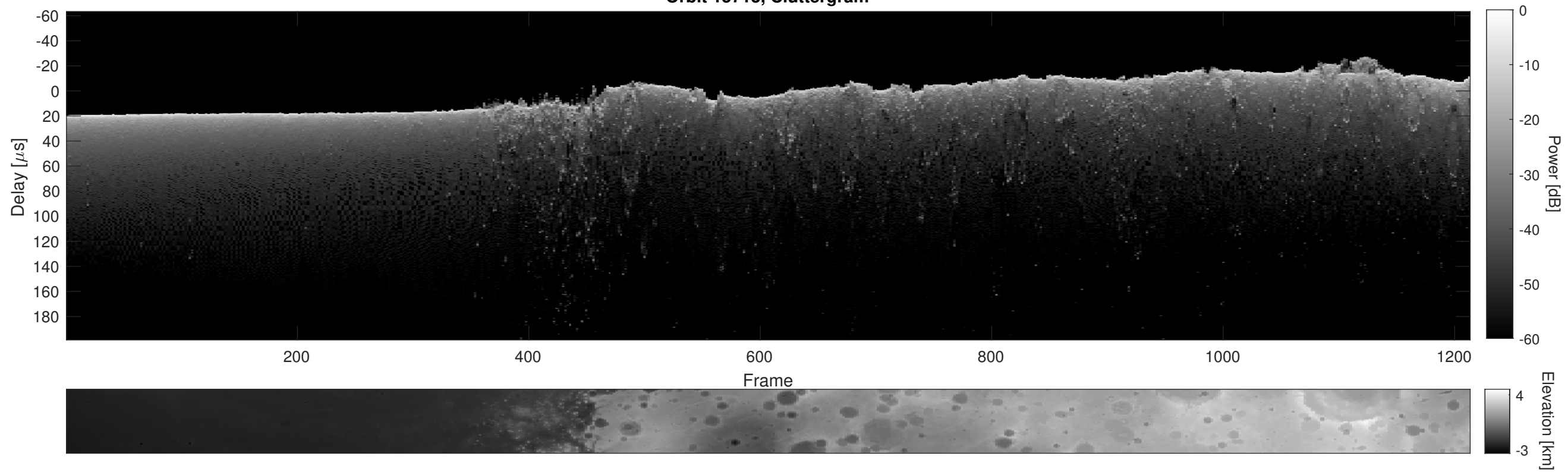
Orbit 15713, Cluttergram
