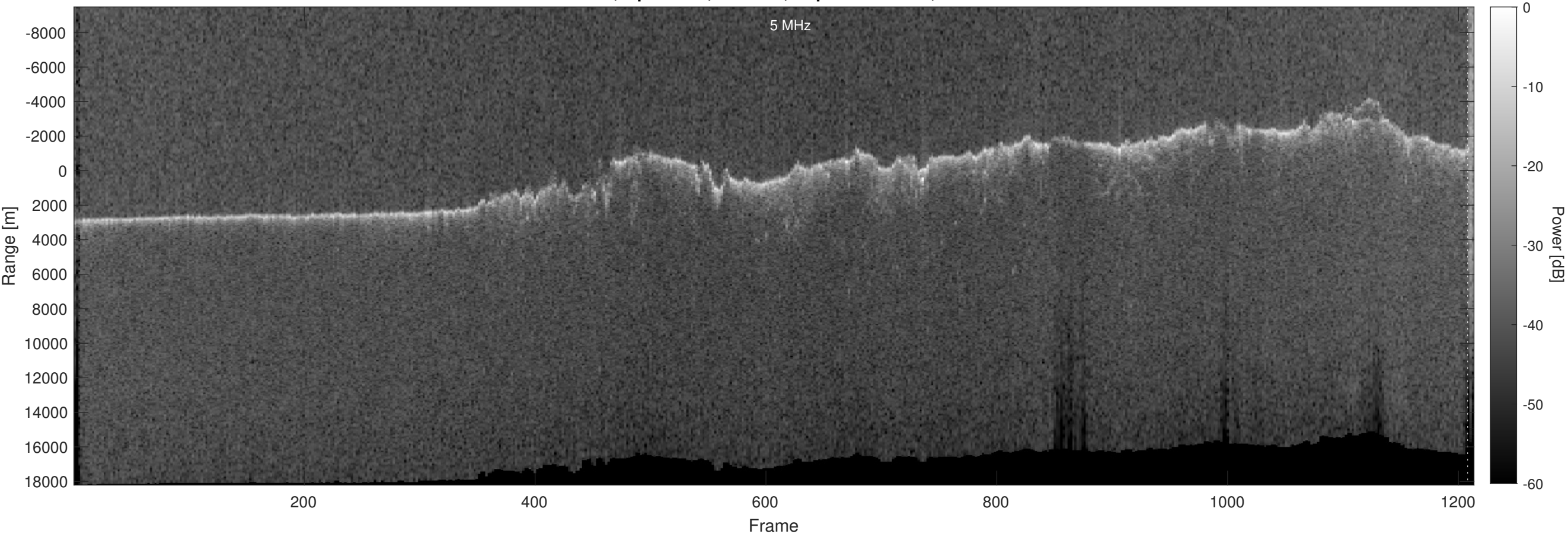
Orbit 15713, Optimized, Window, Depth-Corrected, Channel 2
