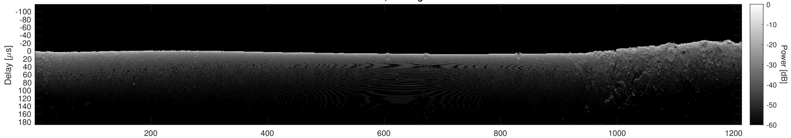
Orbit 15715, Cluttergram
