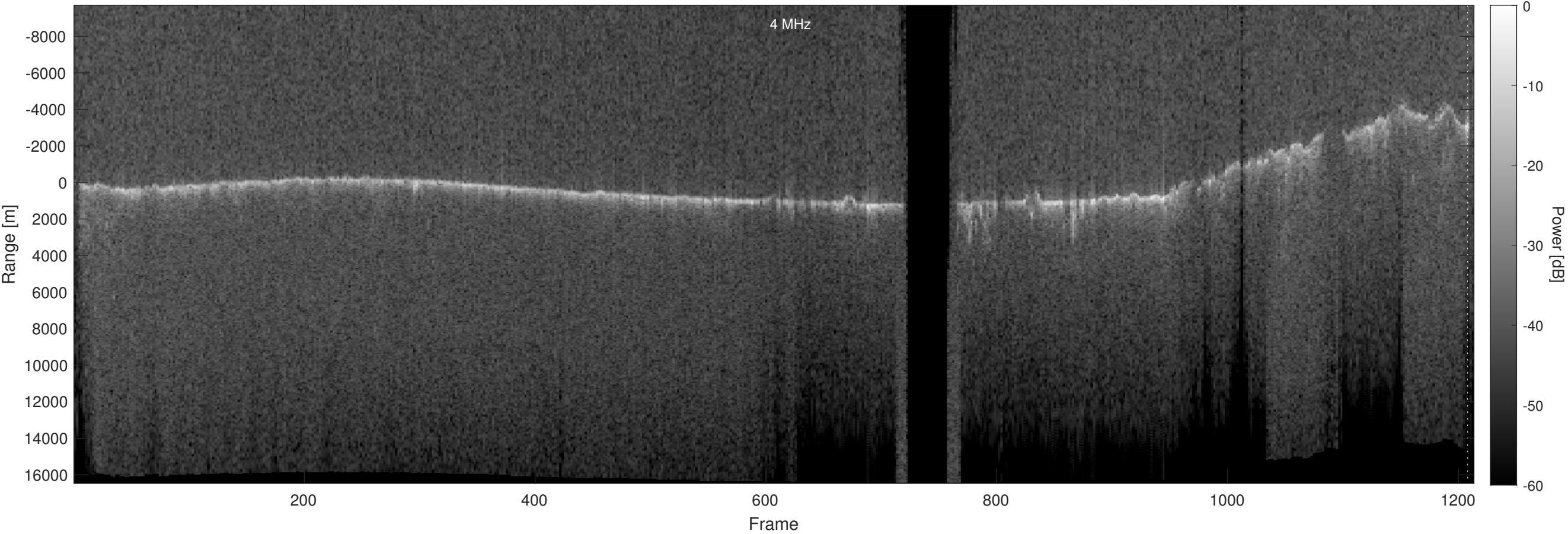
Orbit 15715, Optimized, No Window, Depth-Corrected, Channel 2
