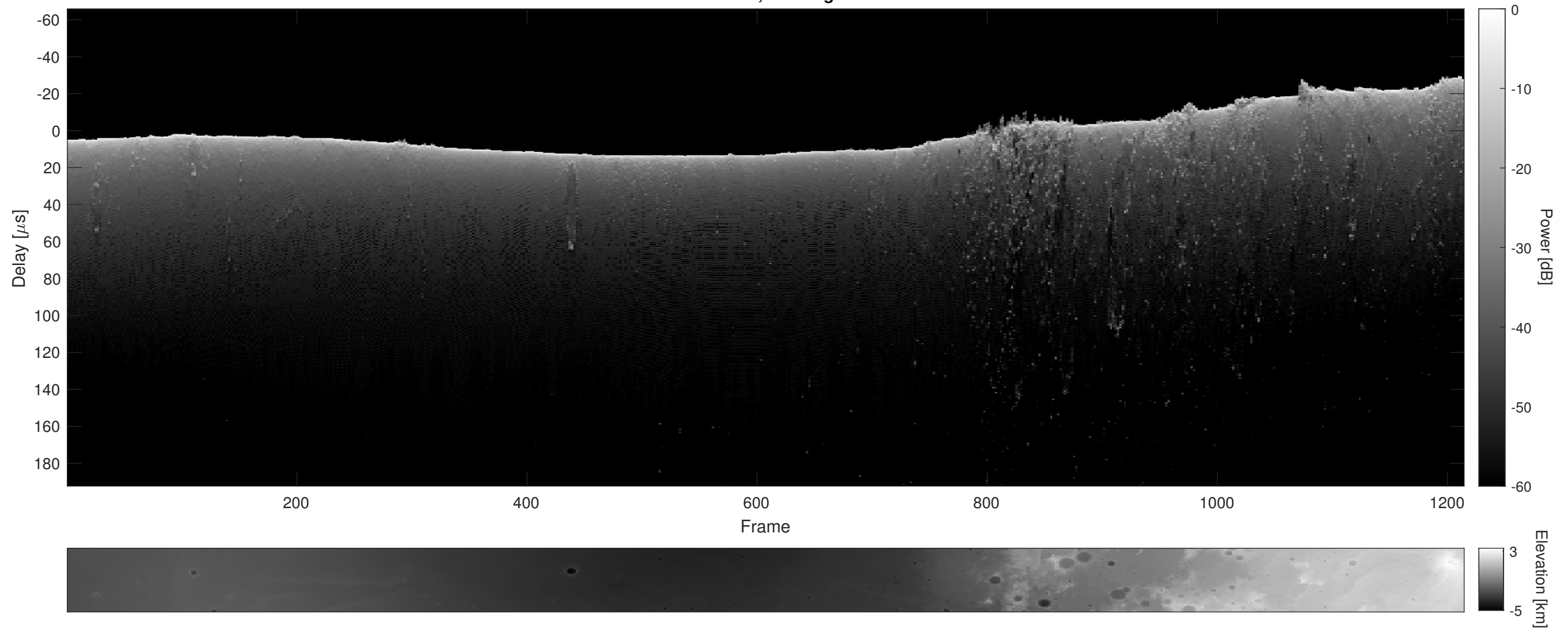
Orbit 15716, Cluttergram
