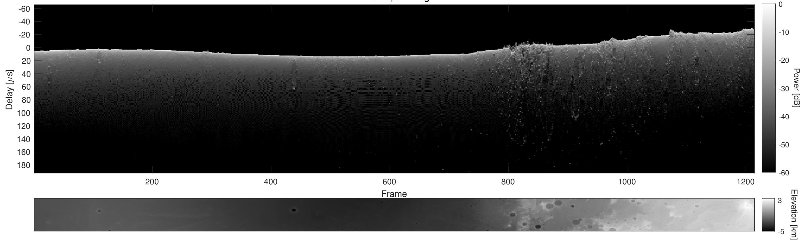
Orbit 15716, Cluttergram
