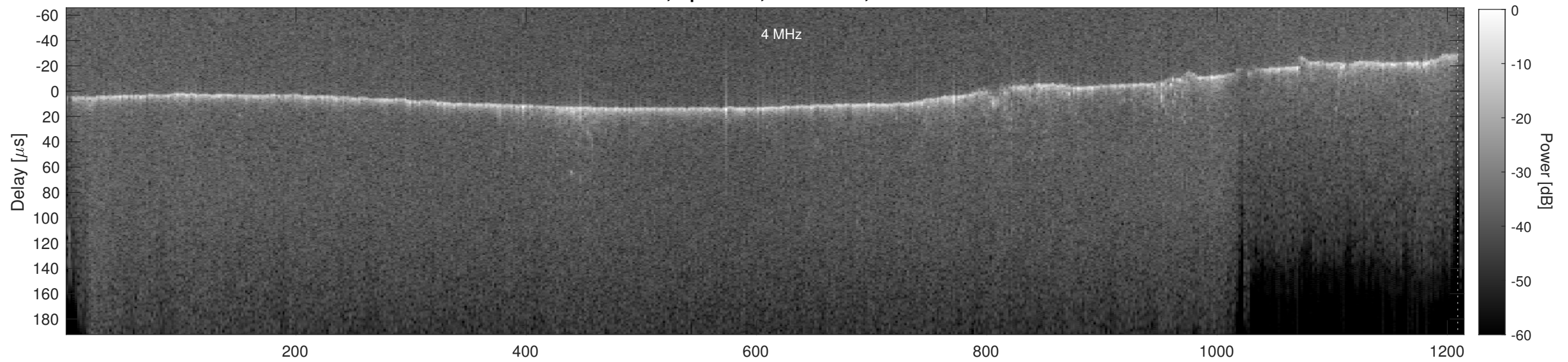
Orbit 15716, Cluttergram
