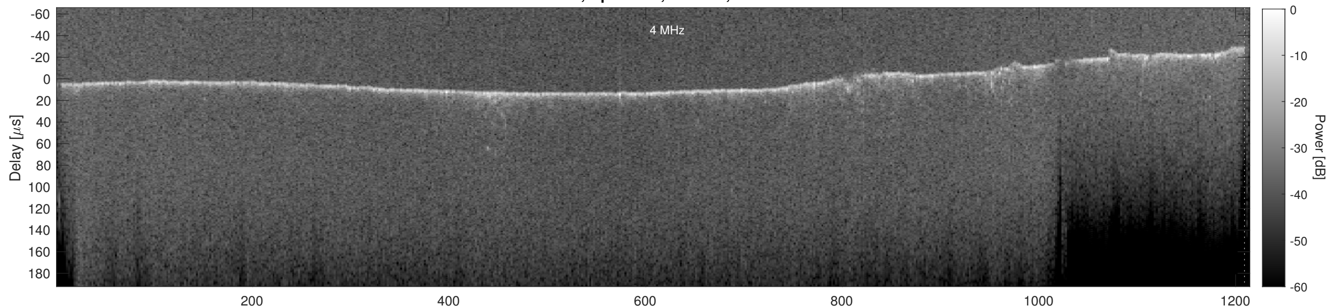
Orbit 15716, Cluttergram
