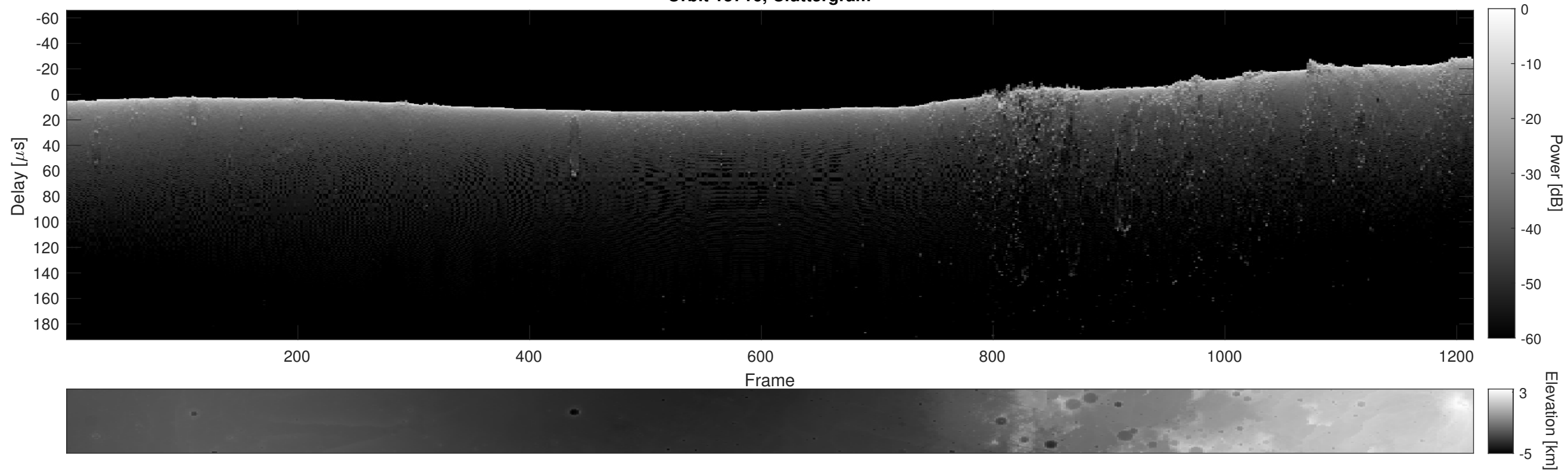
Orbit 15716, Cluttergram
