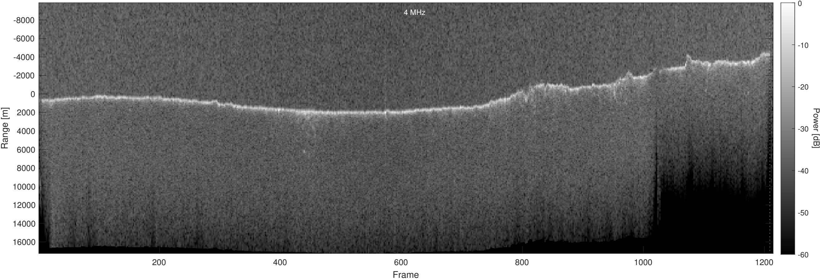
Orbit 15716, Optimized, Window, Depth-Corrected, Channel 2
