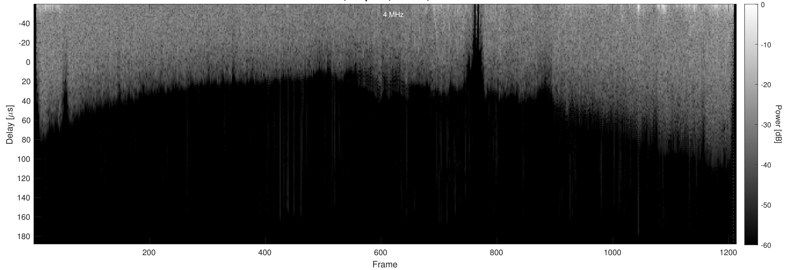
Orbit 15717, Chapman, Window, Channel 2
