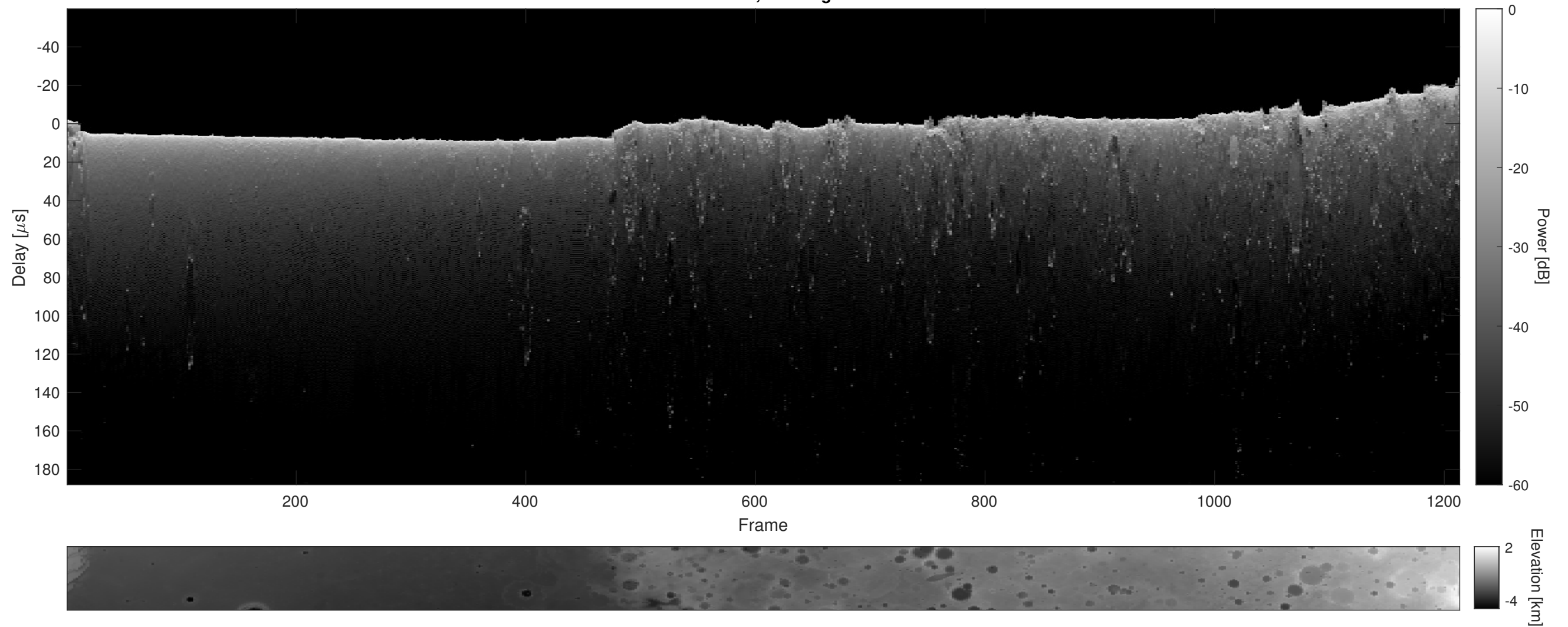
Orbit 15717, Cluttergram
