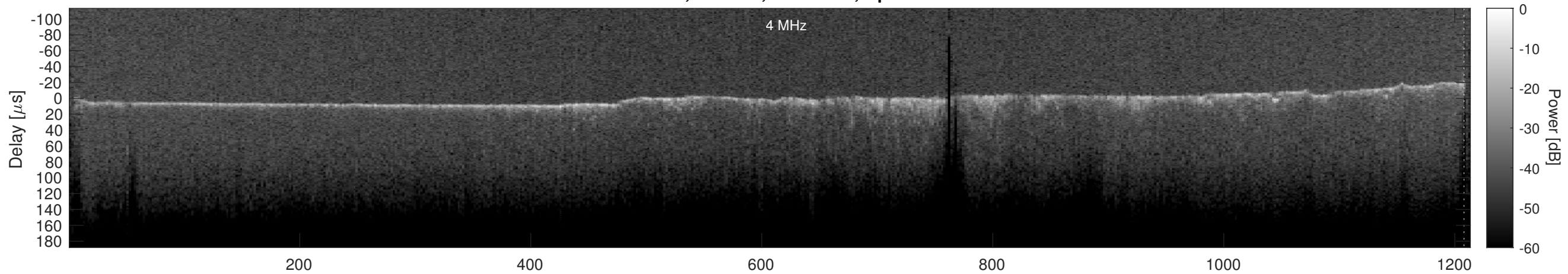
Orbit 15717, Cluttergram
