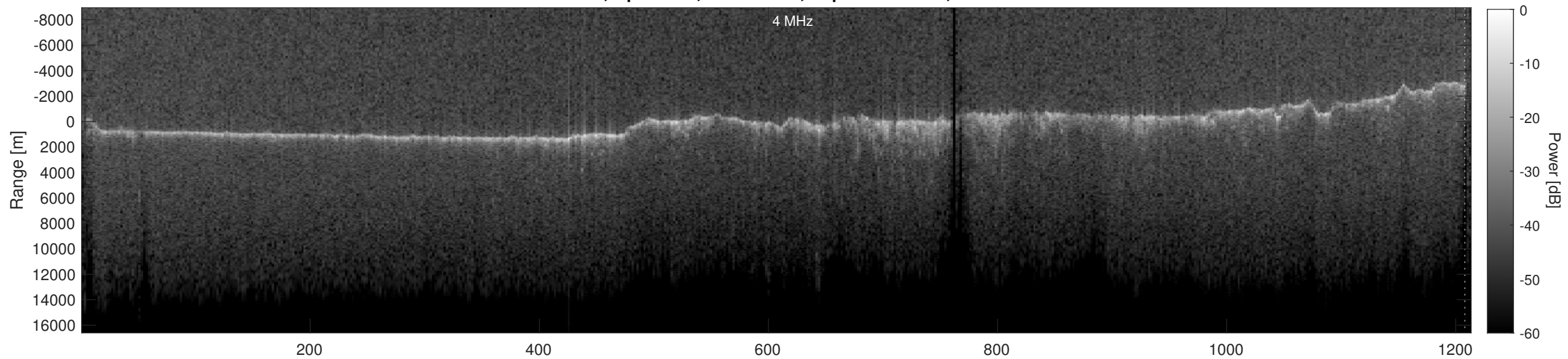
Orbit 15717, Depth-Corrected Cluttergram
