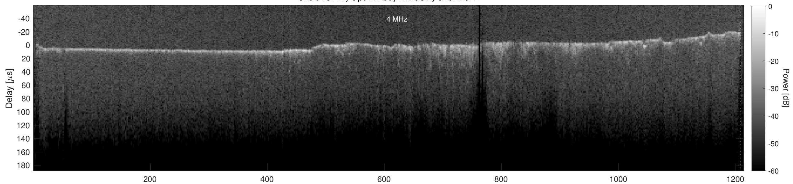
Orbit 15717, Cluttergram
