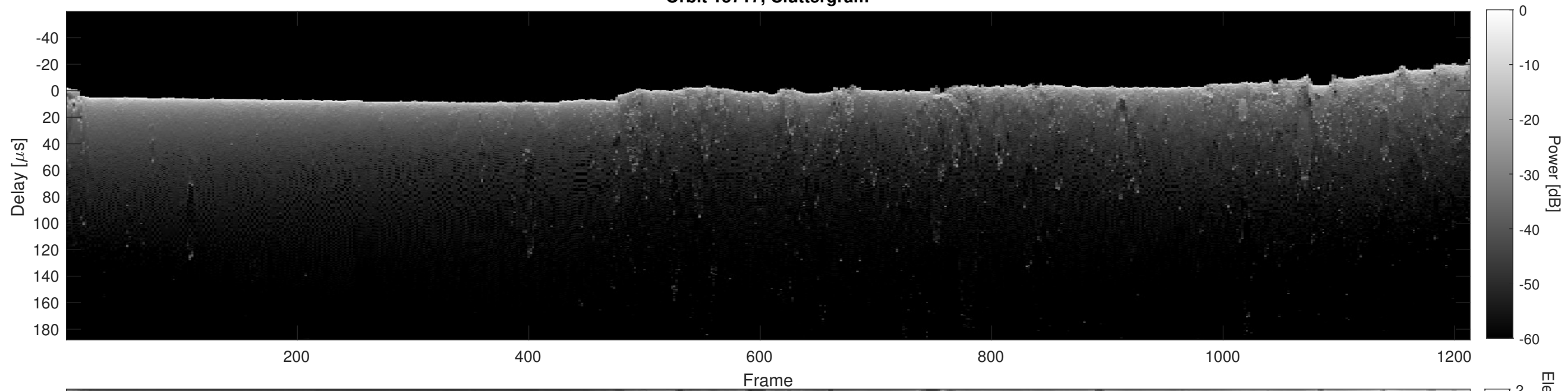
Orbit 15717, Cluttergram
