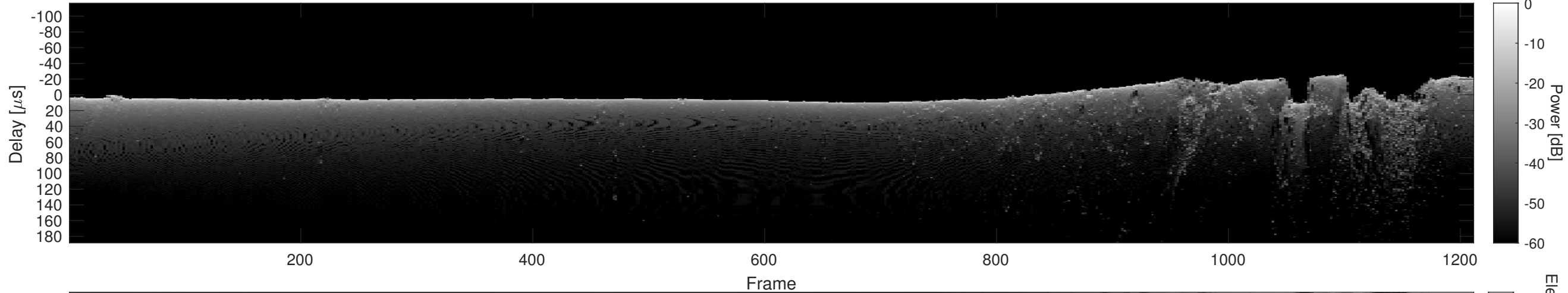
Orbit 15721, Cluttergram
