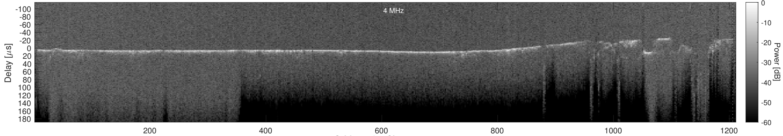
Orbit 15721, Cluttergram
