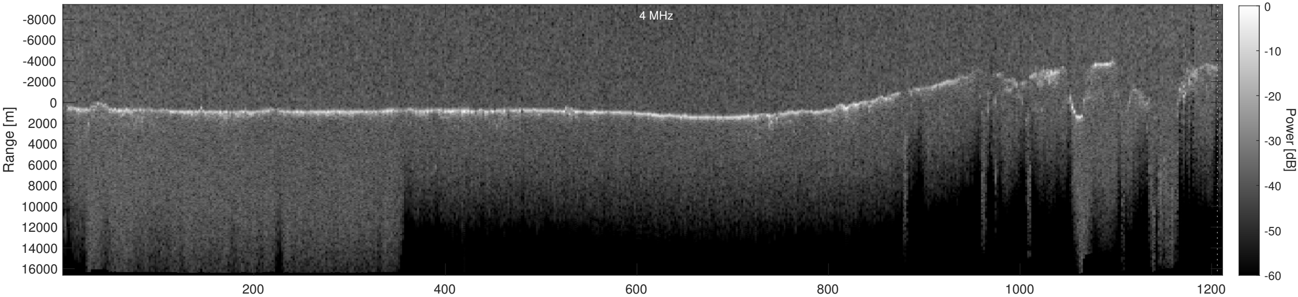
Orbit 15721, Depth-Corrected Cluttergram
