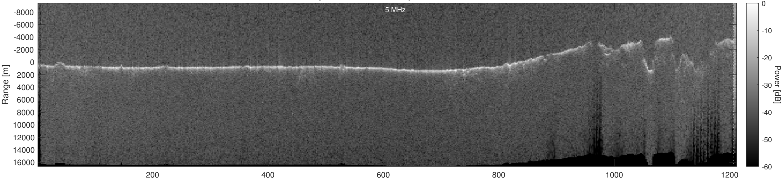
Orbit 15721, Optimized, Window, Depth-Corrected, Channel 2
