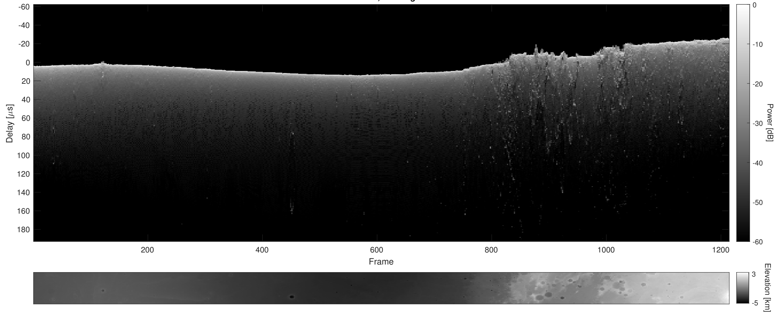
Orbit 15723, Cluttergram
