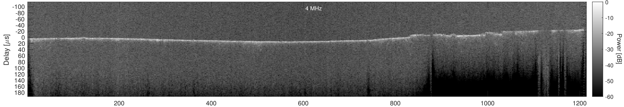
Orbit 15723, Cluttergram
