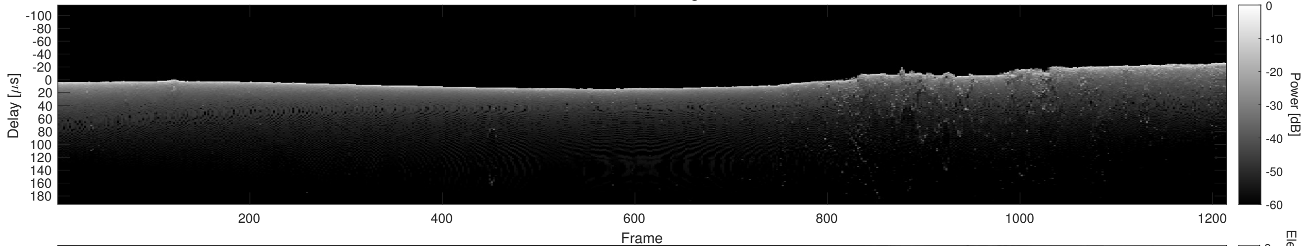
Orbit 15723, Cluttergram
