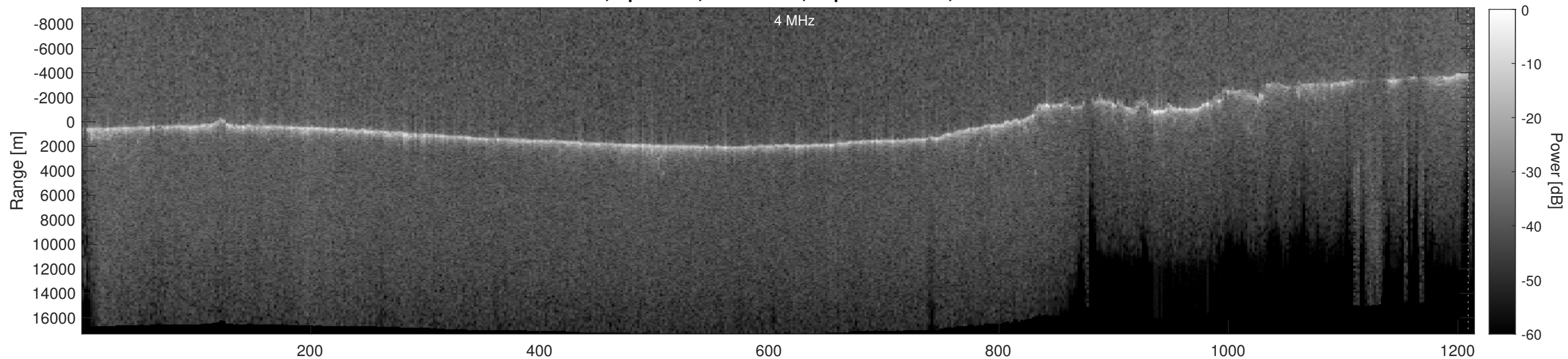
Orbit 15723, Depth-Corrected Cluttergram
