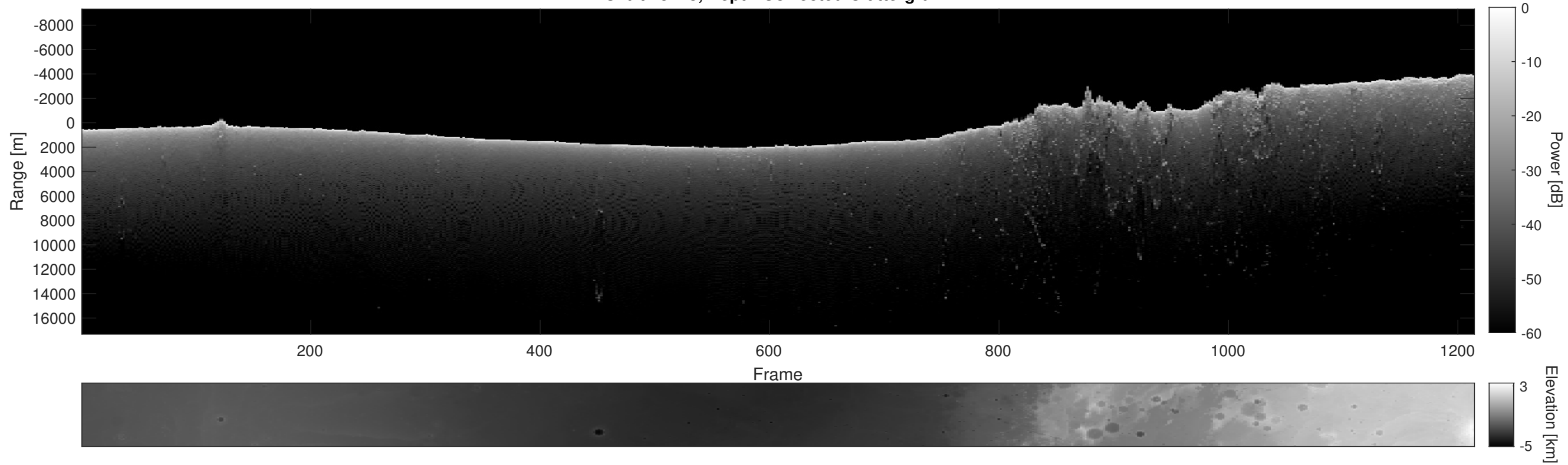
Orbit 15723, Depth-Corrected Cluttergram
