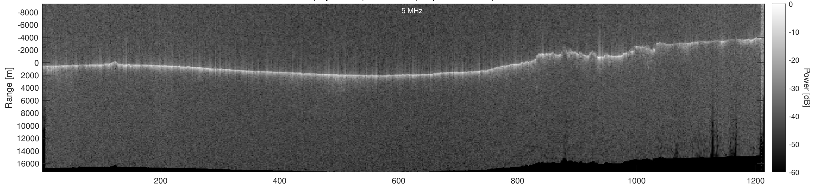
Orbit 15723, Optimized, No Window, Depth-Corrected, Channel 2
