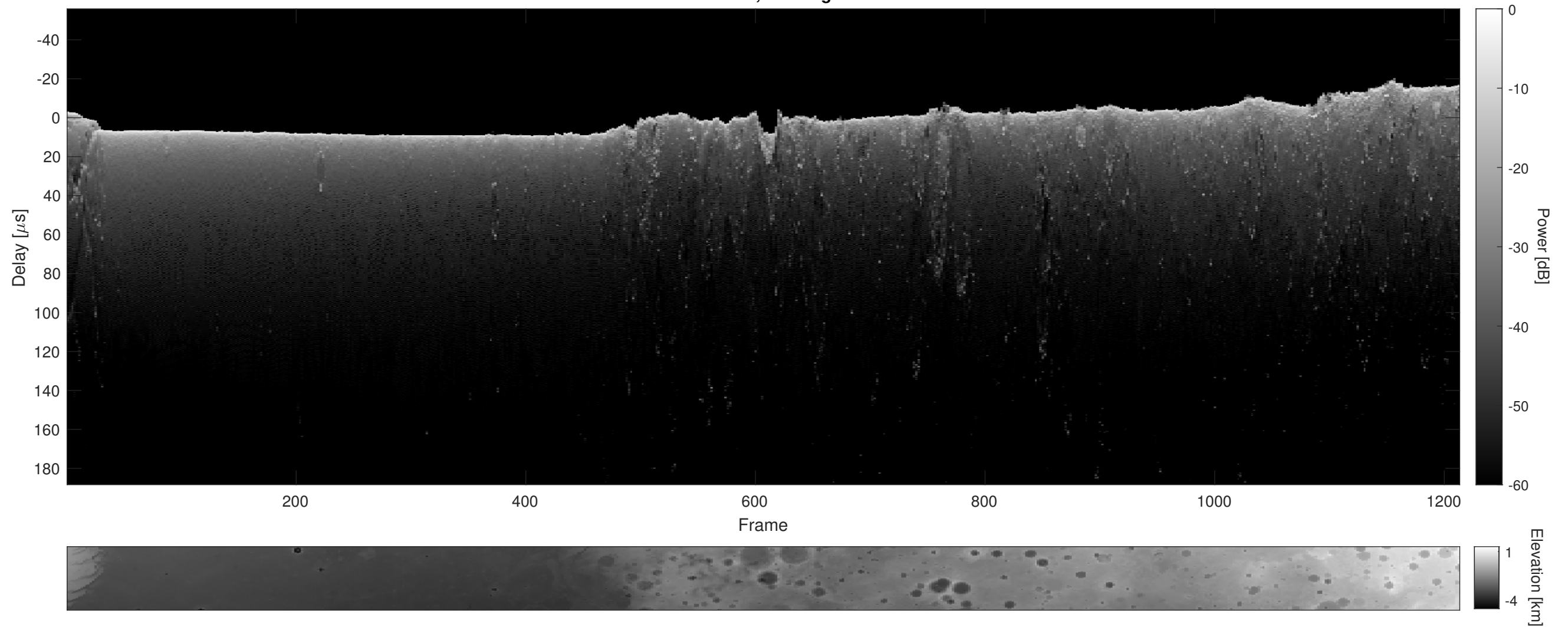
Orbit 15724, Cluttergram
