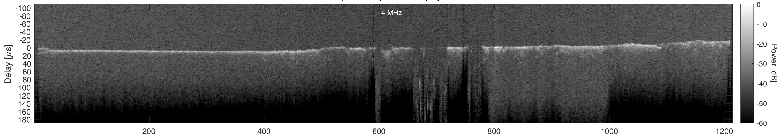
Orbit 15724, Cluttergram
