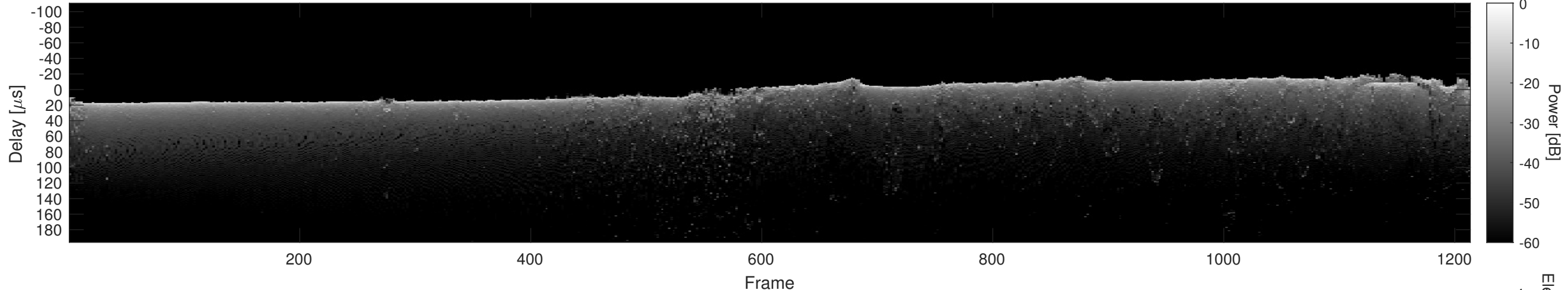
Orbit 15727, Cluttergram
