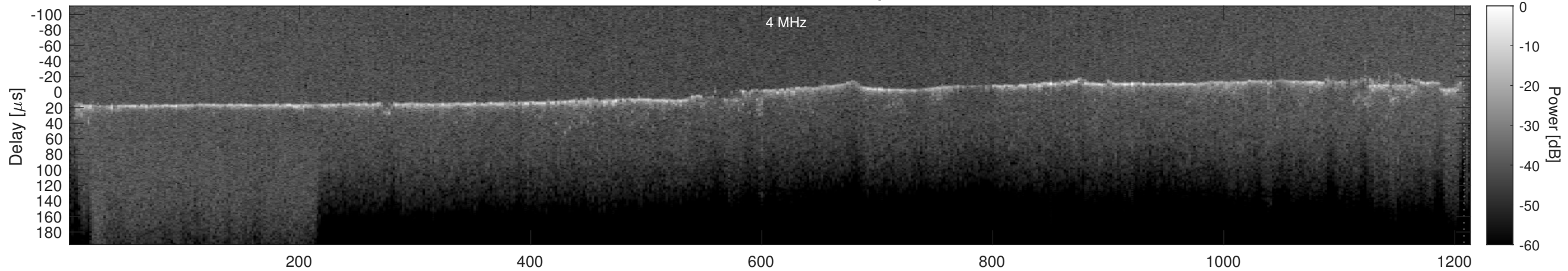
Orbit 15727, Cluttergram
