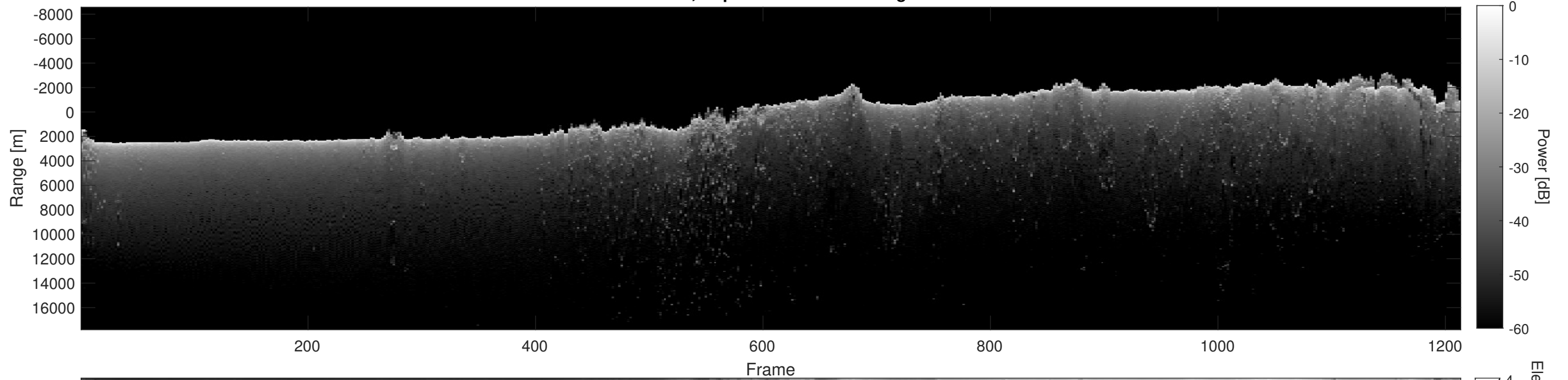
Orbit 15727, Depth-Corrected Cluttergram
