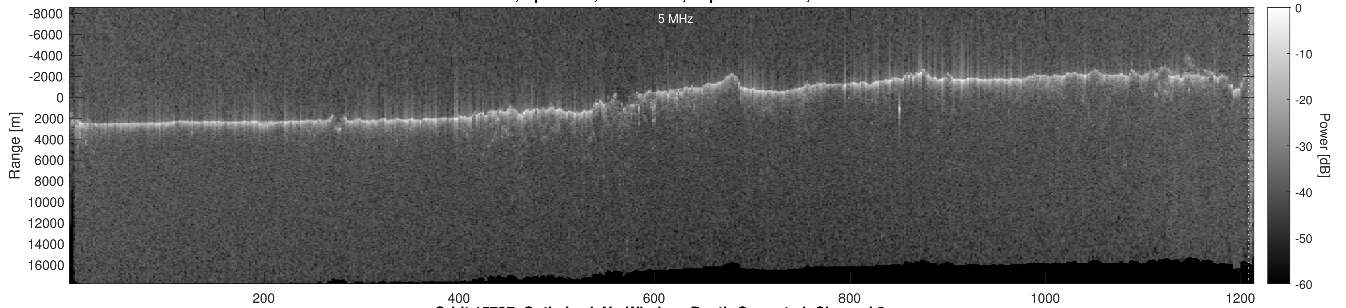
Orbit 15727, Optimized, No Window, Depth-Corrected, Channel 2
