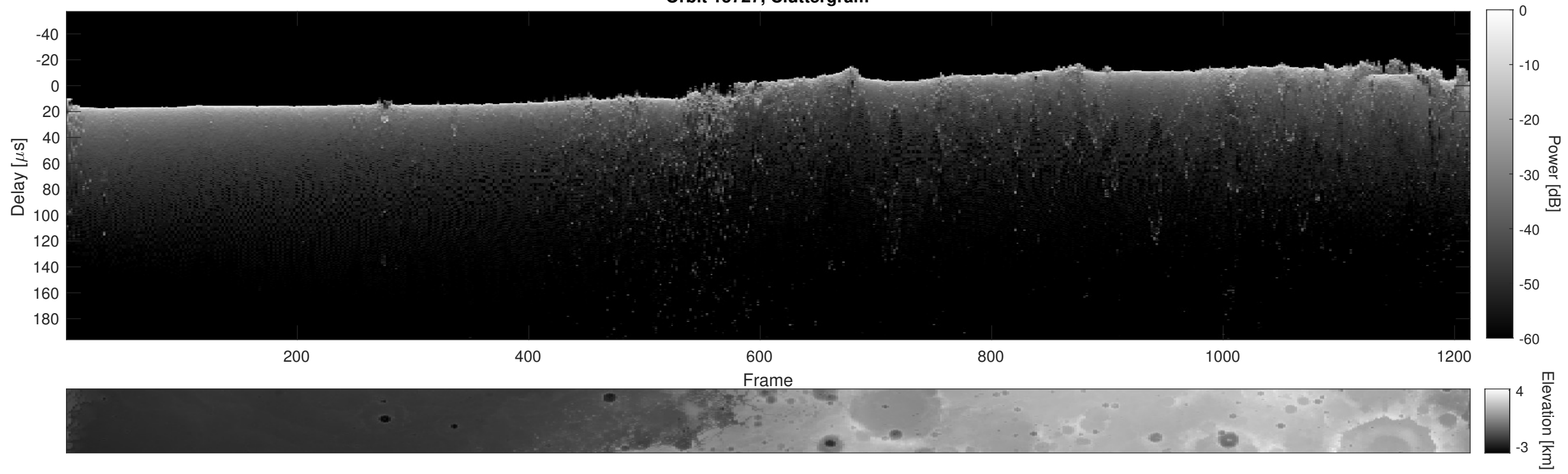
Orbit 15727, Cluttergram
