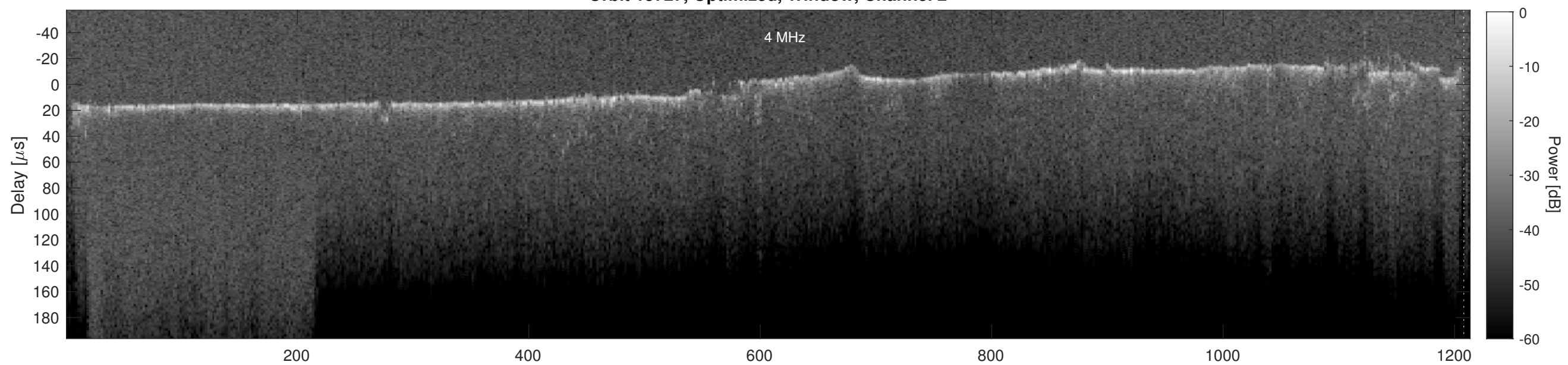
Orbit 15727, Cluttergram
