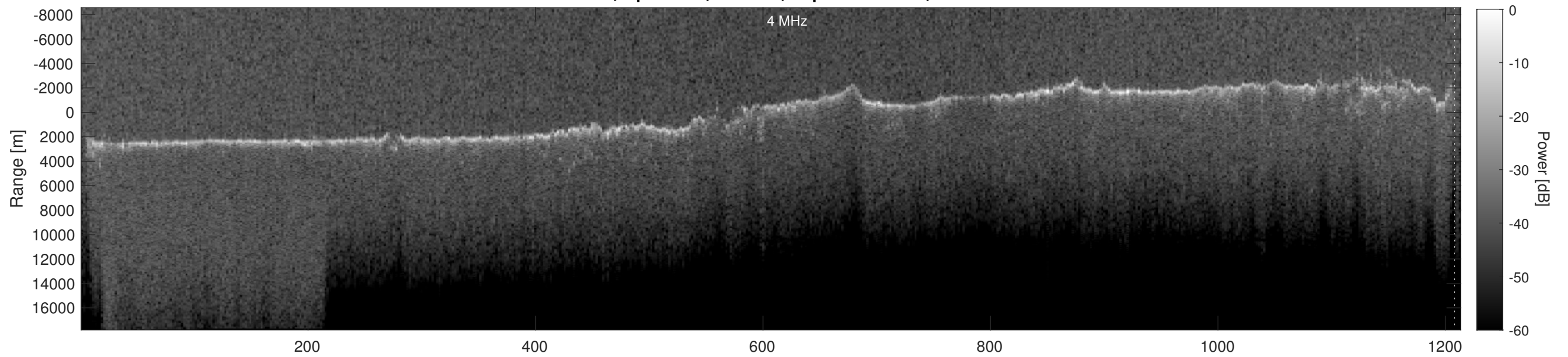
Orbit 15727, Depth-Corrected Cluttergram
