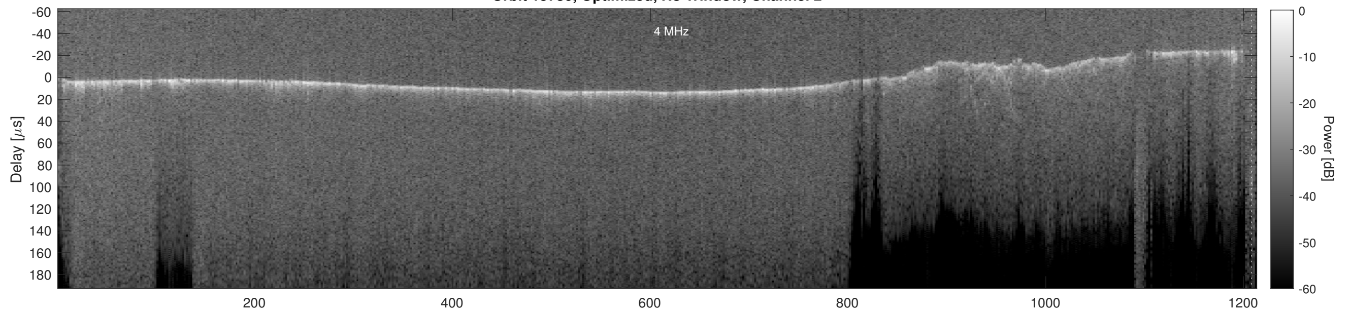
Orbit 15730, Cluttergram
