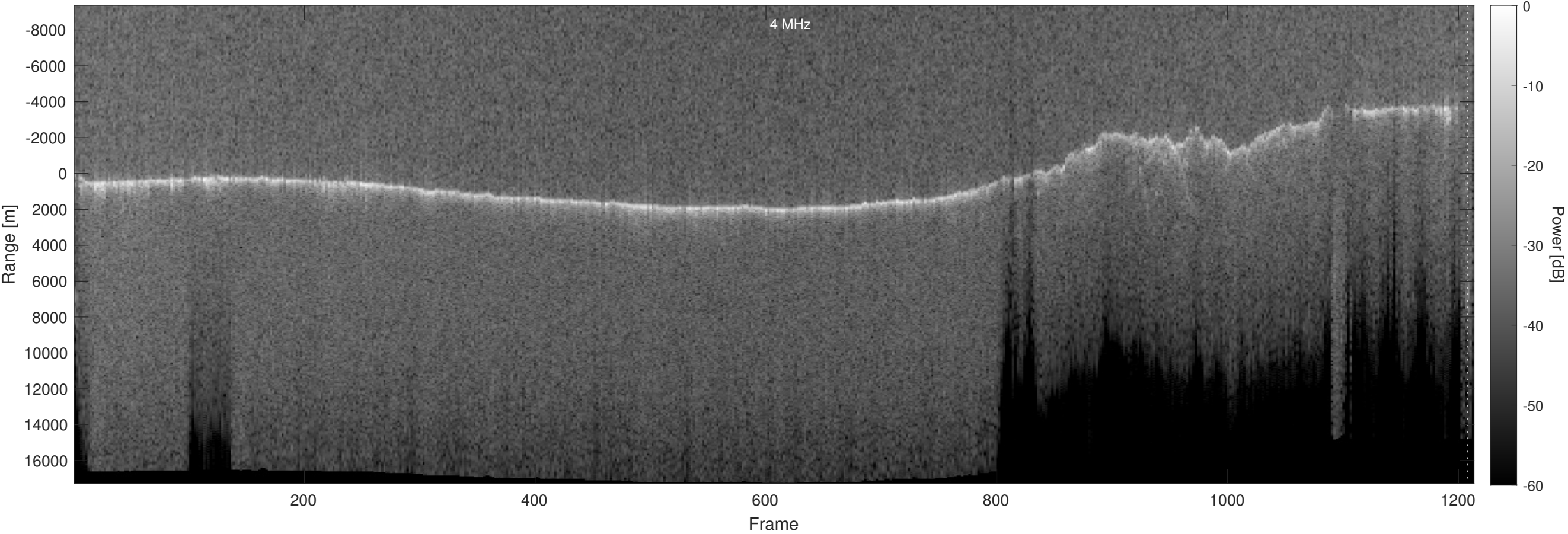
Orbit 15730, Optimized, No Window, Depth-Corrected, Channel 2
