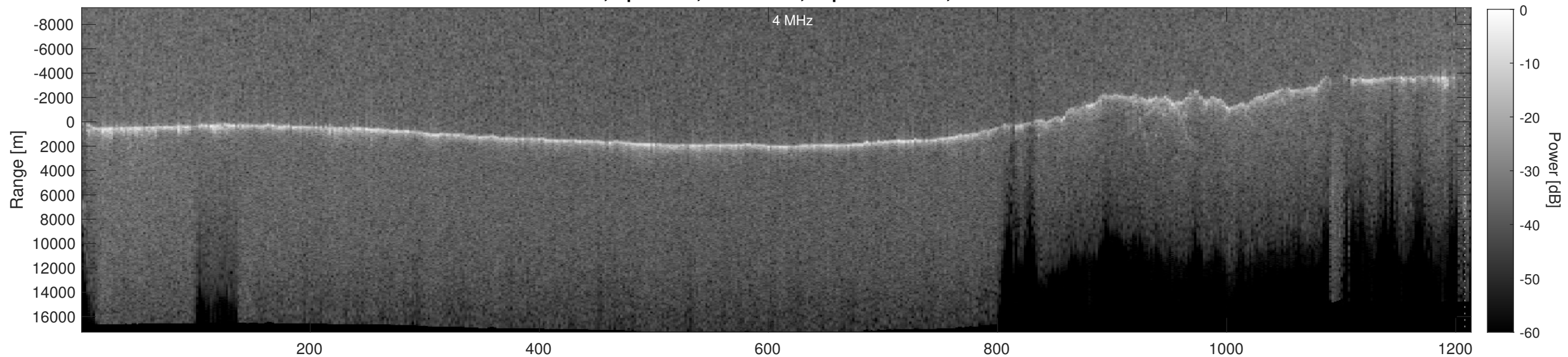
Orbit 15730, Depth-Corrected Cluttergram
