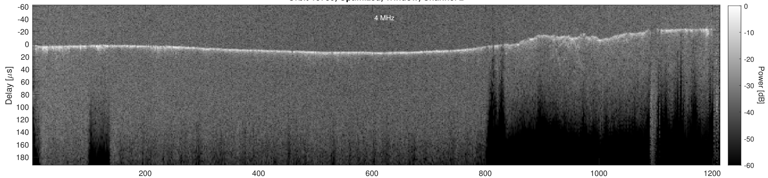
Orbit 15730, Cluttergram
