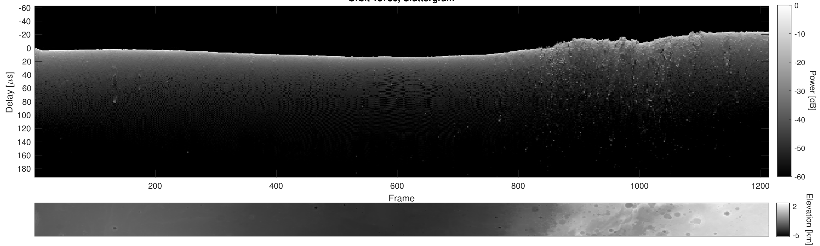
Orbit 15730, Cluttergram
