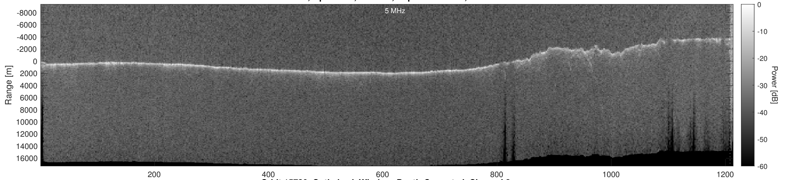
Orbit 15730, Optimized, Window, Depth-Corrected, Channel 2
