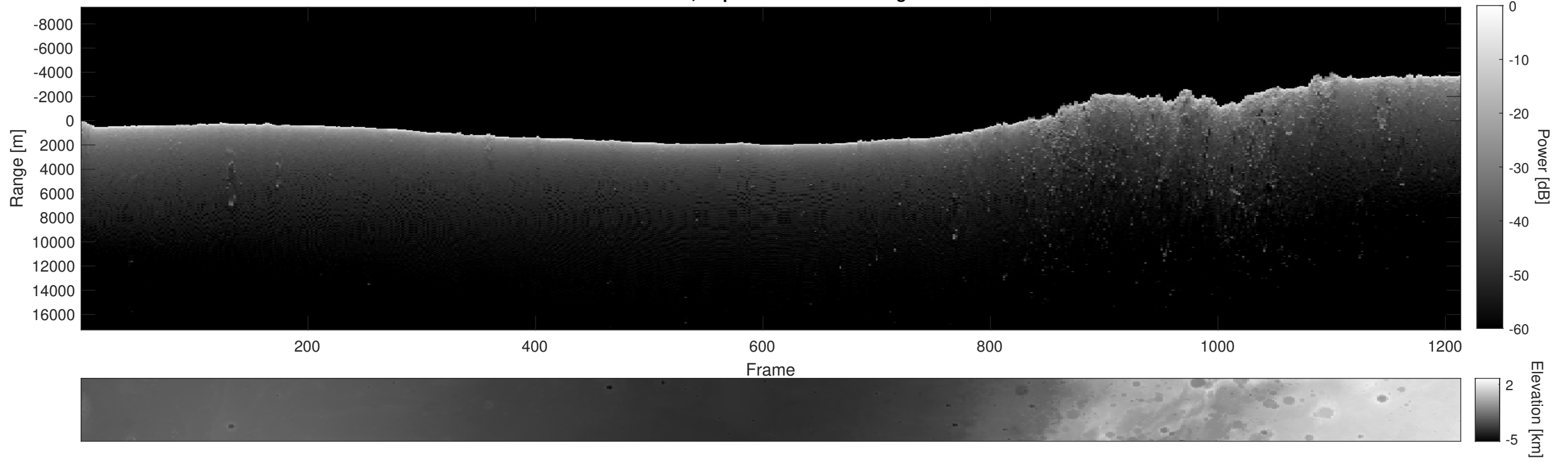
Orbit 15730, Depth-Corrected Cluttergram
