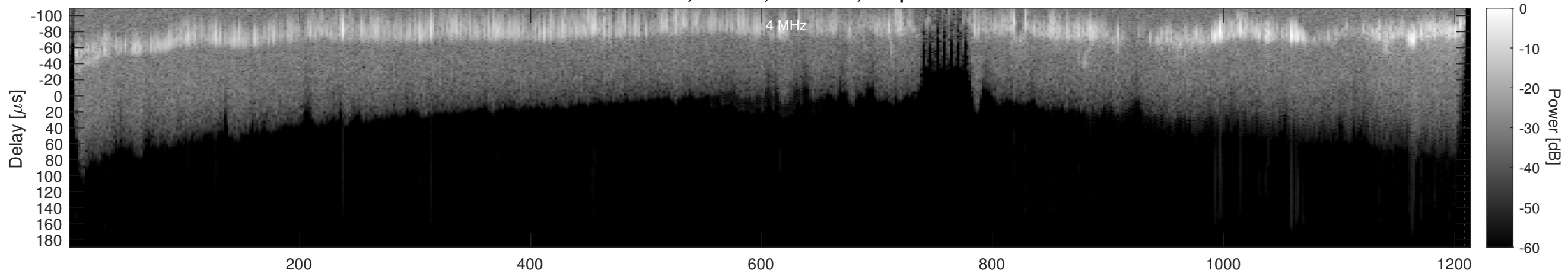
Orbit 15731, Window, Channel 2, Optimized
