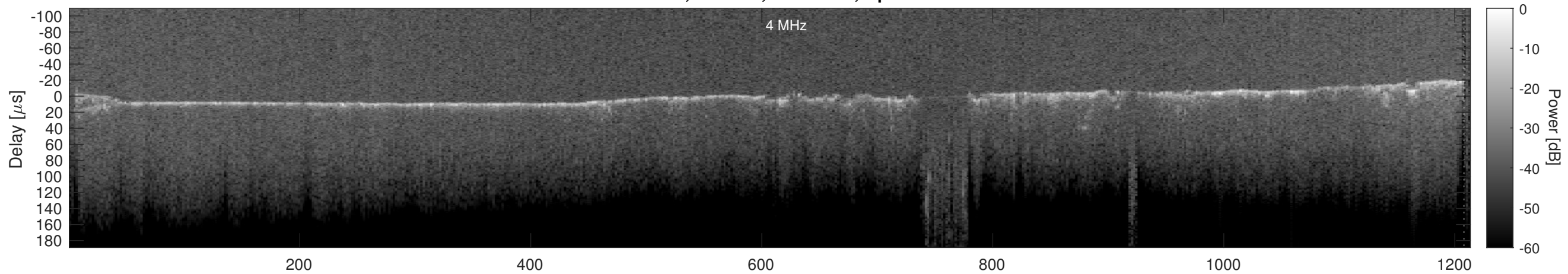
Orbit 15731, Cluttergram
