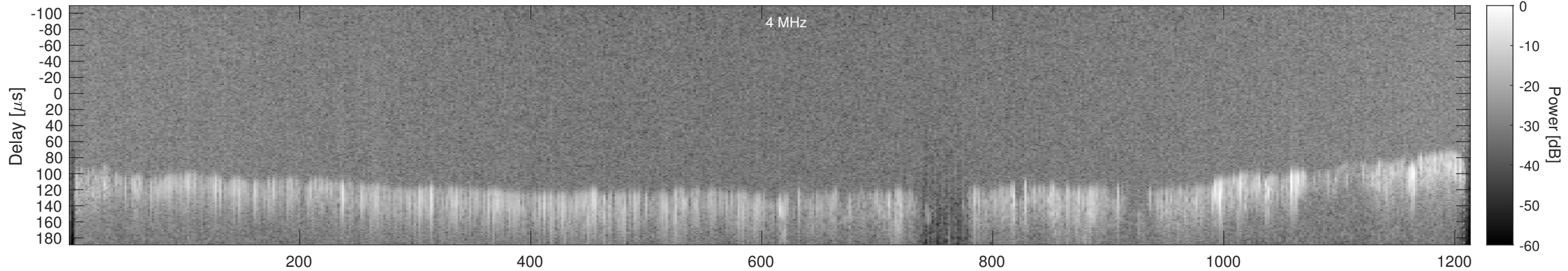
Orbit 15731, Window, Channel 2, Chapman
