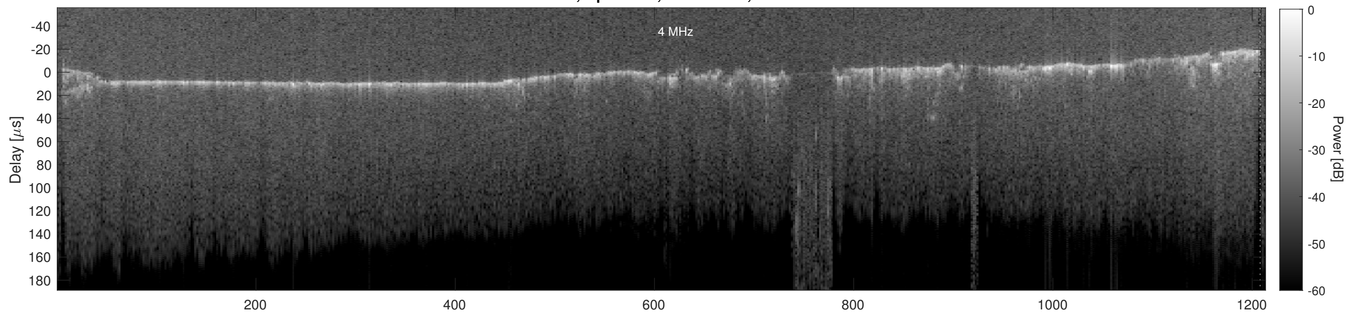
Orbit 15731, Cluttergram
