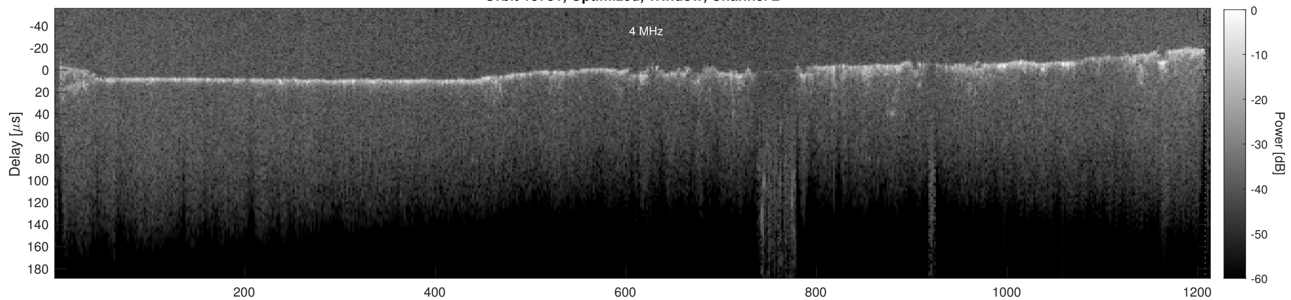
Orbit 15731, Cluttergram
