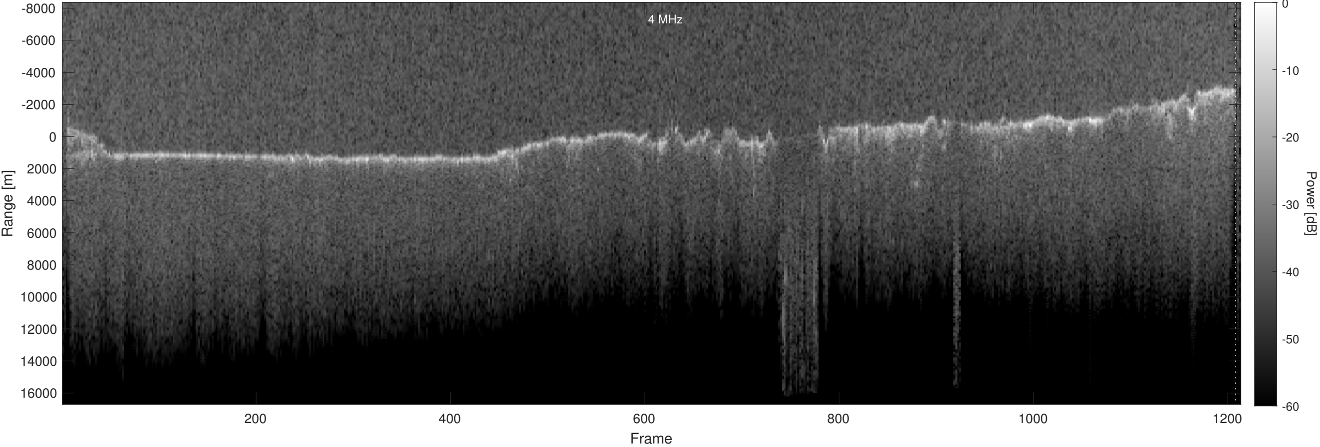
Orbit 15731, Optimized, Window, Depth-Corrected, Channel 2
