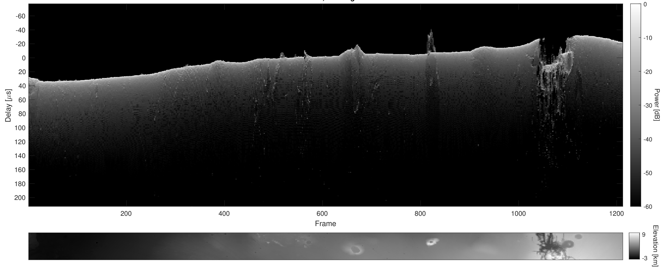
Orbit 15732, Cluttergram
